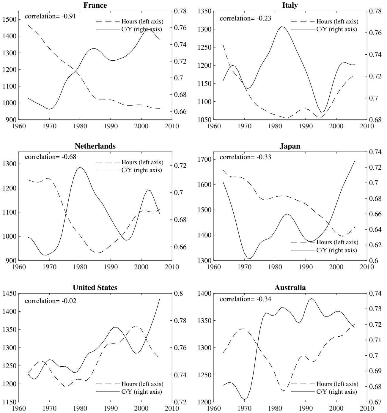
Figure 4: Trend Hours and Trend Consumption-Output Ratio (HP: 6.25)
