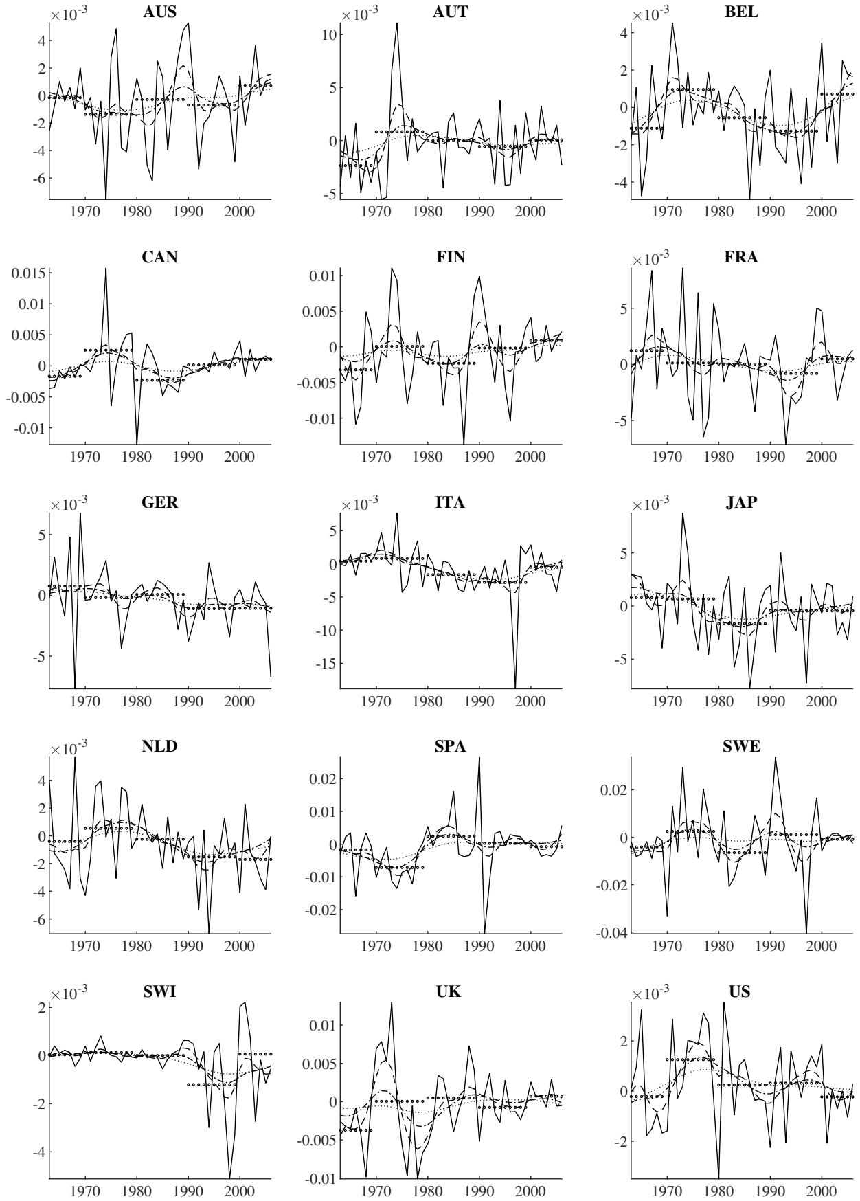
Figure 12: Tax Wedge \tau^{cx} (solid: data, dashed HP 6.25, dashed-dotted HP 62.5, dotted HP 625, circles: decade means)
