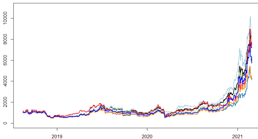
Fig. 1: Scaled CC indices: BBGCI , Bitwise 10 , CCI30 , CRIX , F5 , HODL5 , and the total market index (TMI, black solid line). The indices deviate from the TMI due to methodological differences in their construction. evaluation_indices
