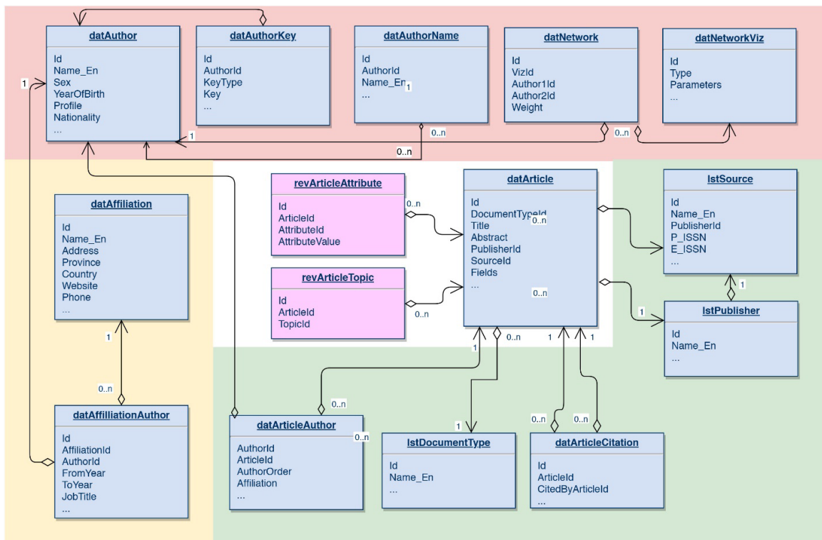
Figure 4. The data structure of SSHPA and SDA.
