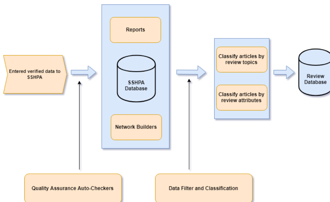
Figure 3. The workflow of SSHPA and SDA systems.
