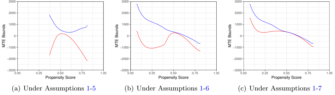
Figure 2: Unconditional Bounds around the MTE^{OO}
