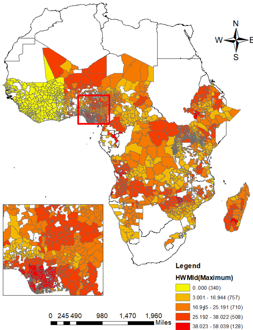
Figure 1: Maximum heat wave magnitudes by district (1979–2016)
