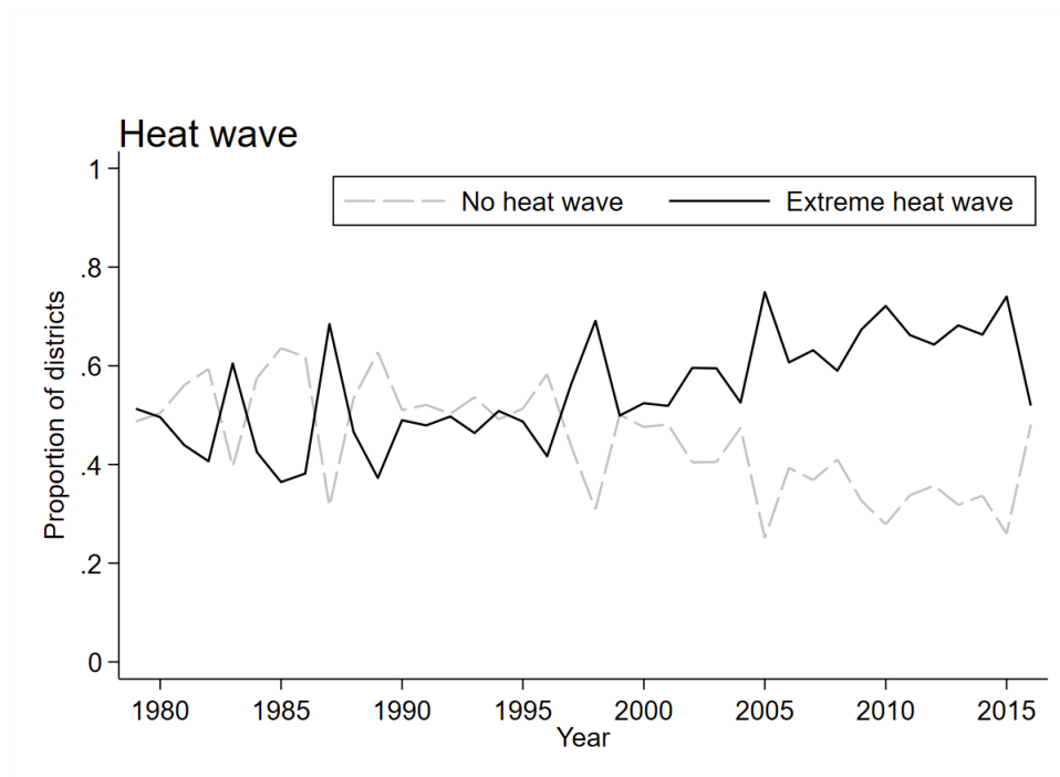
Figure 2: Trend of heat waves in Sub-Saharan Africa
