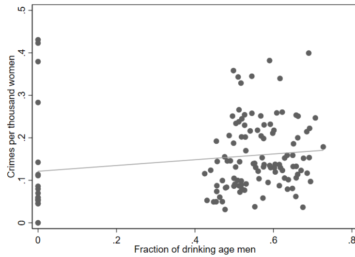
Figure 6: First-stage Correlation
