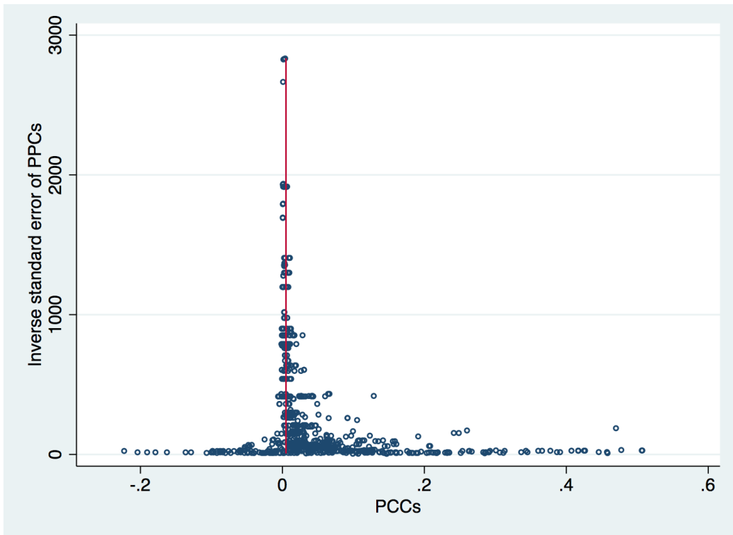
Figure 2: Funnel-Asymmetry Plot
