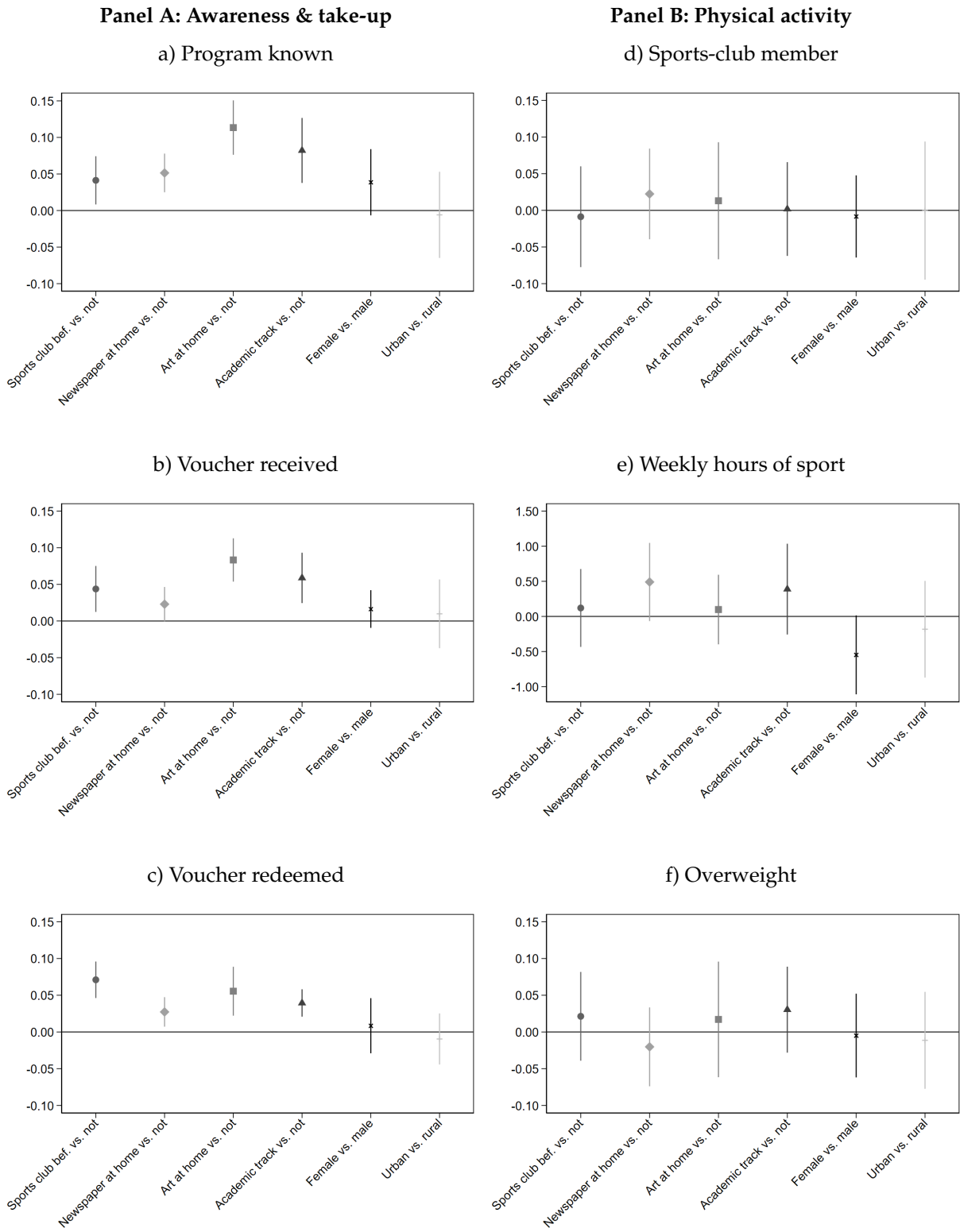
Figure 2: Effect Heterogeneity
