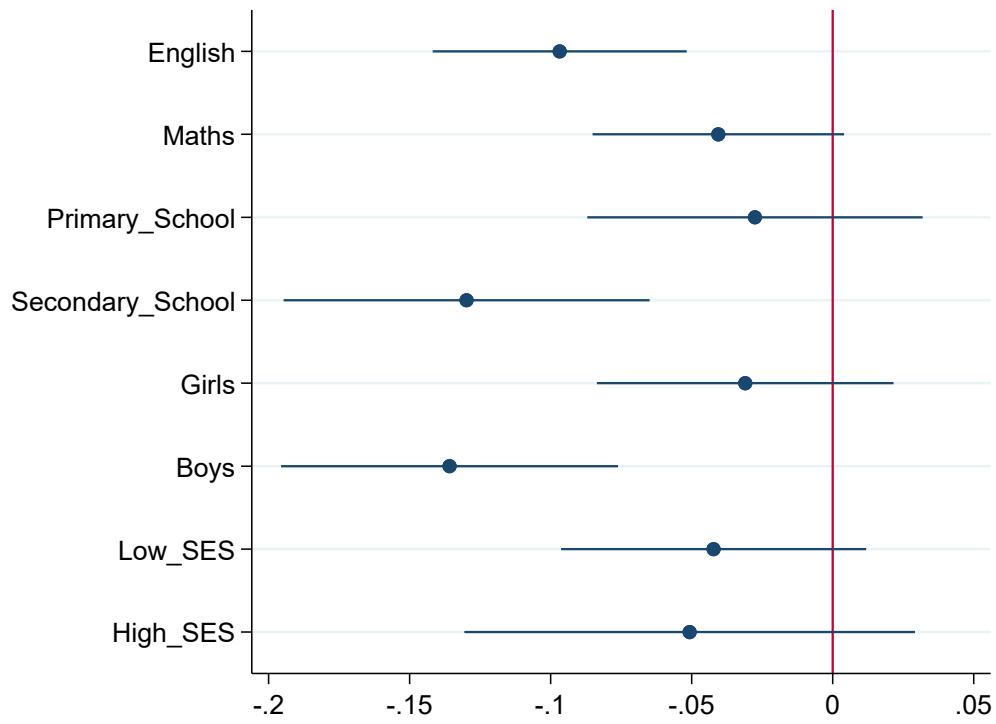
Figure 2 – Heterogeneity Analysis
