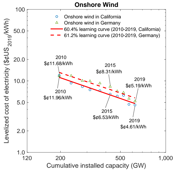
Figure 8: LCOE Dynamics: Wind Power
