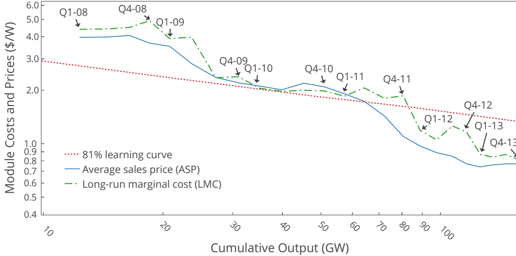
Figure 3: Average sales prices and long-run marginal costs of solar PV modules (Reichelstein and Sahoo, 2018).
