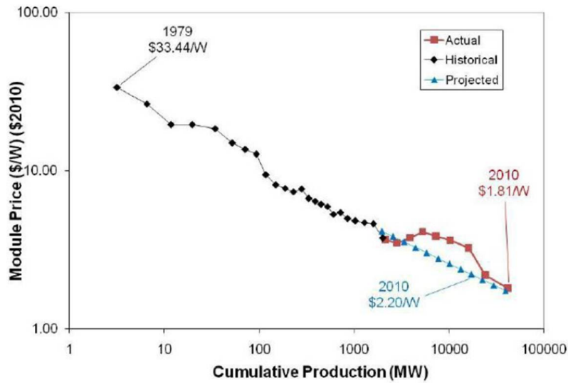
Figure 1: Historic solar PV module prices (Swanson, 2011).
