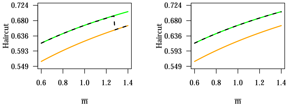
Figure 7: Varying uncertainty about a continuous belief set ranging from \underline{m} = 0.5 to \overline{m} .
