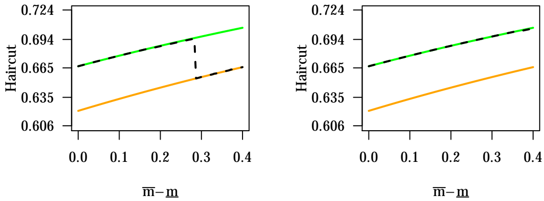
Figure 6: Varying uncertainty about a continuous belief set ranging from \underline{m} to \overline{m} symmetrically centered around one.
