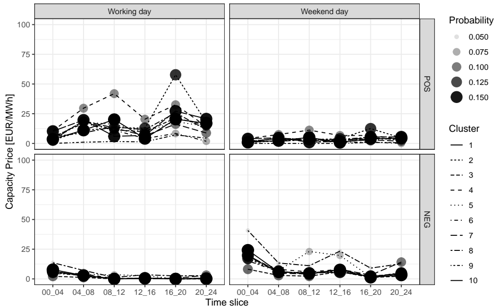
Figure 14: Scenarios derived from the stochastic modelling for the transition season on medium levels of PV generation and residual load, distinguished by reserve product and type of weekday. Reserve price scenarios for typeday tra2 correspond to the left column.
