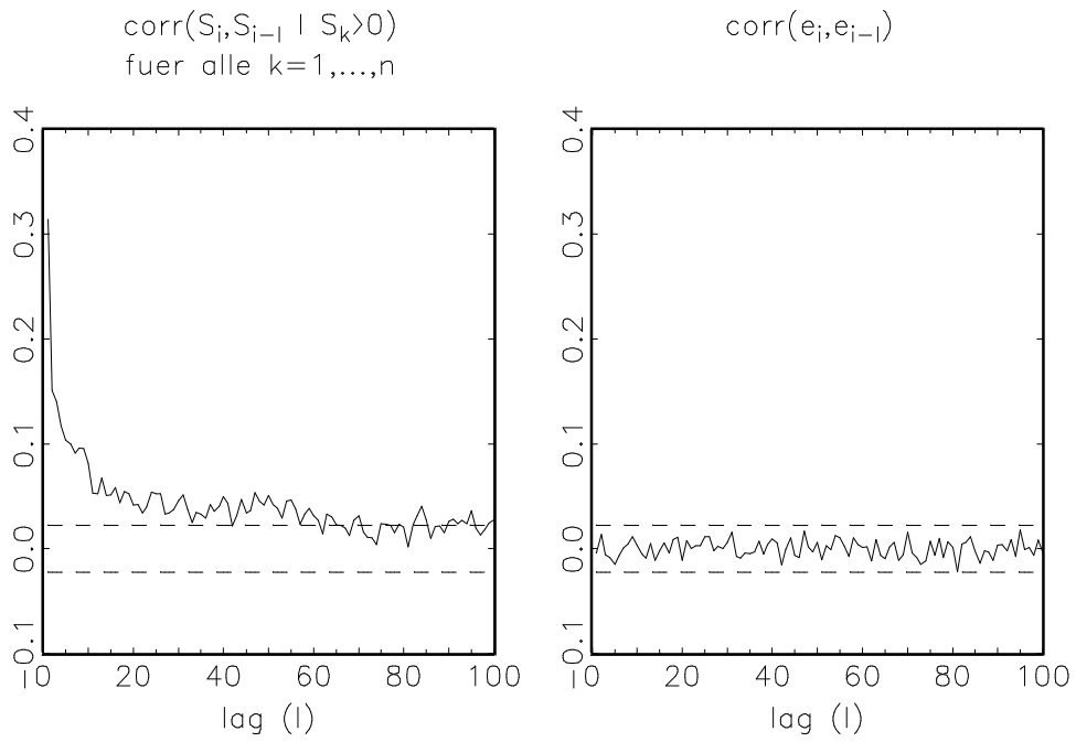
Figure 4: Auto correlation function of the non-zero absolute transaction price changes S_i \mid S_i > 0 (left) and the standardized residuals e_i of the asymmetric GLARMA(2,3)-model (right). The dashed lines mark off the approximative 99% confidence interval \pm 2.58/\sqrt{\tilde{n}} , where \tilde{n} the number of non-zero price changes.
