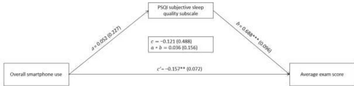
Figure 1. Mediation model
