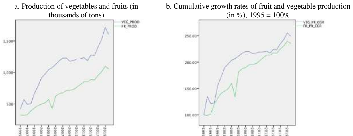
Figure 1: Overall Performance of Fruit and Vegetable Production in Azerbaijan (1991–2020)
