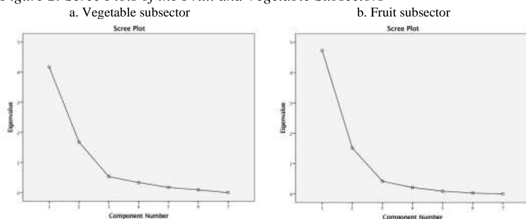
Figure 2: Scree Plots of the Fruit and Vegetable Subsectors
