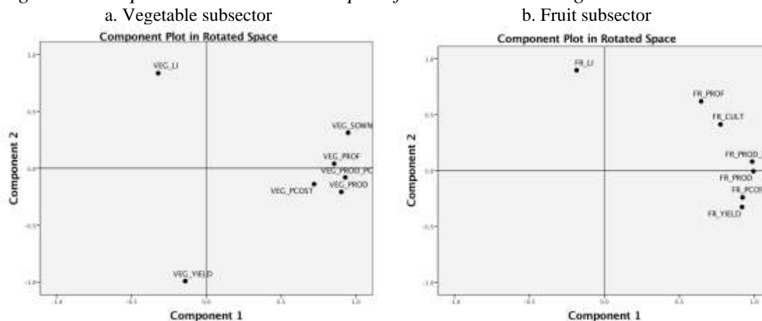
Figure 3: Component Plot in Rotated Space for the Fruit and Vegetable Subsectors
