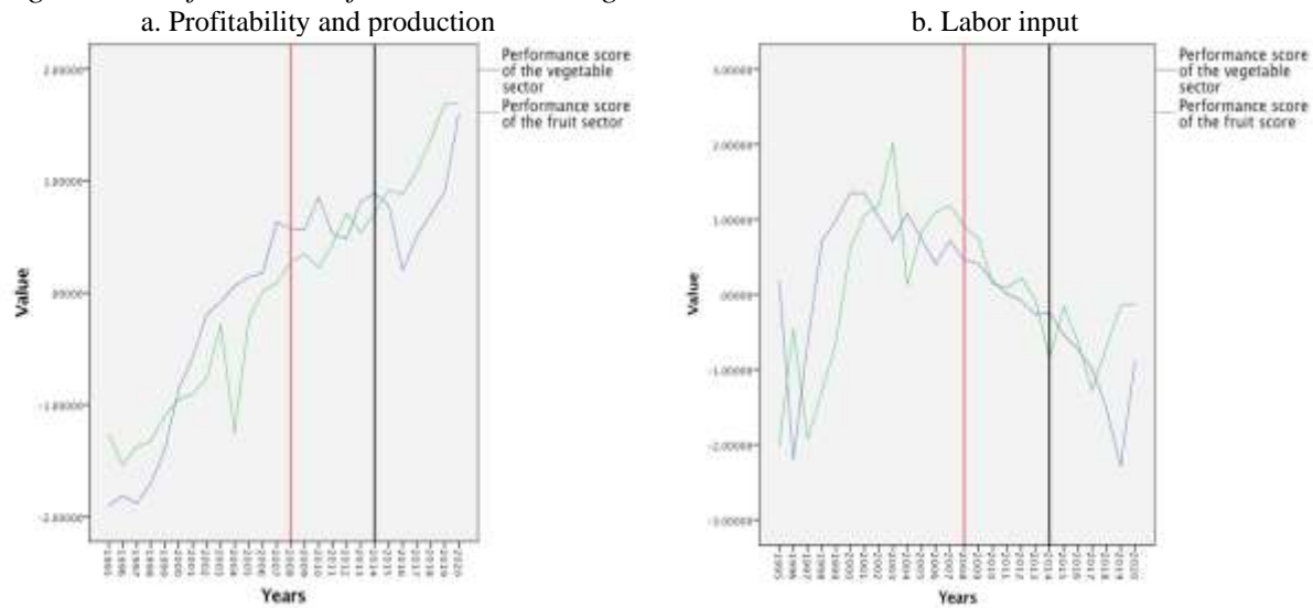
Figure 4: Performance of the Fruit and Vegetable Subsectors Based on Factor Scores
