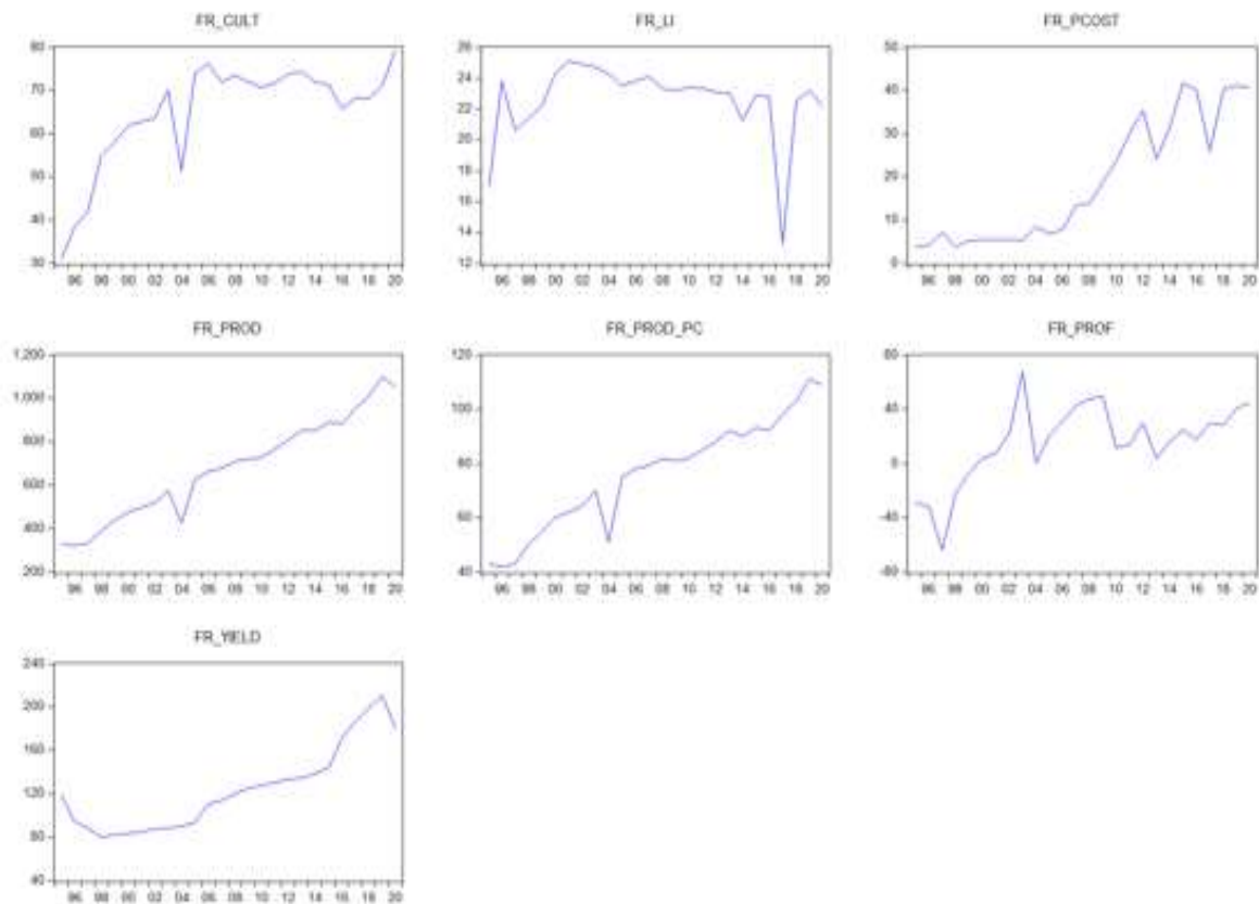
Figure 2A : Fruit Variables.
