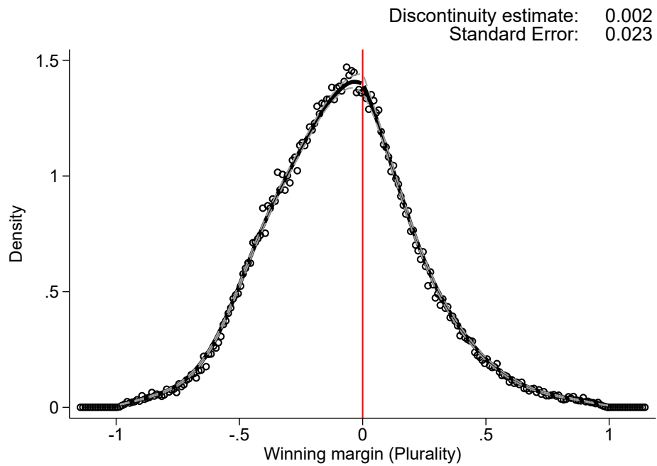
Figure F.1: McCrary (2008) test
