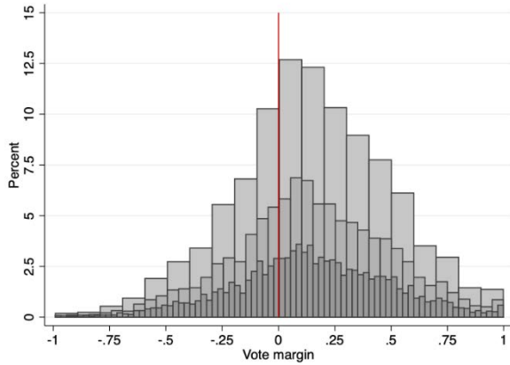
(a) Histogram
