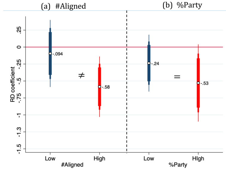
Figure 6: Majority size
