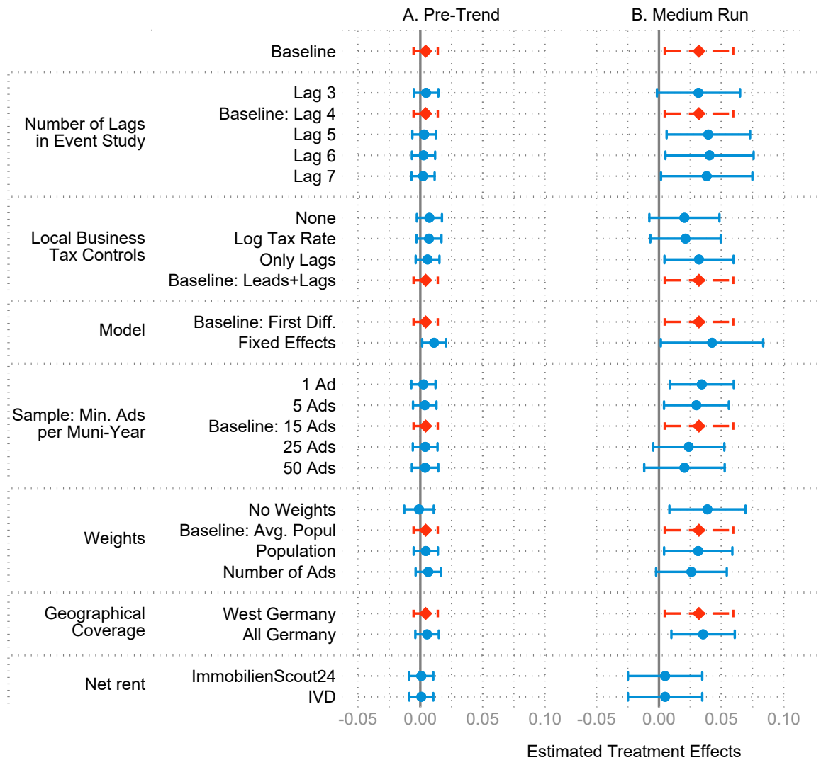
Figure 7: Robustness Checks
