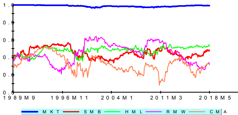
Figure 1: Rolling estimates of factor strength for the five Fama-French factors
