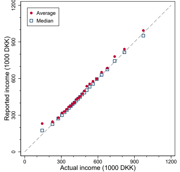
(B) CORRELATION
