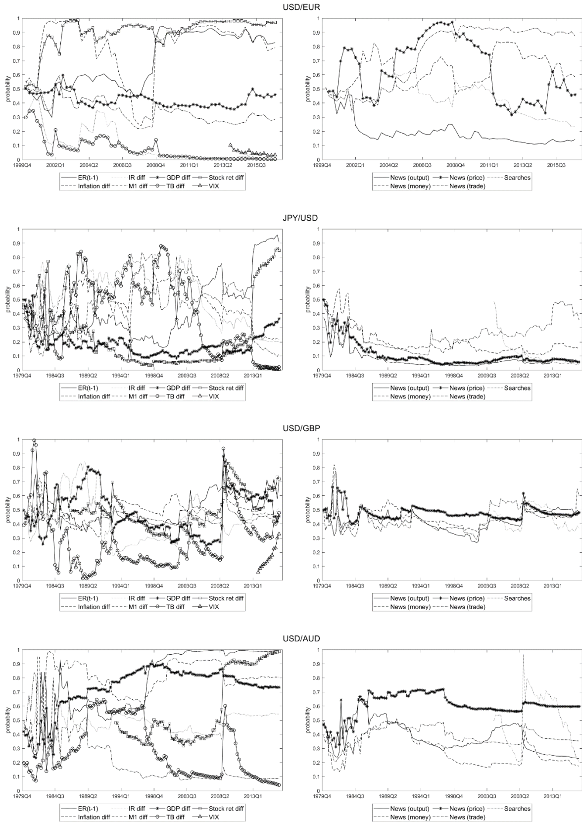
Figure 3. Time-varying posterior probabilities of including predictors into the extended models.
