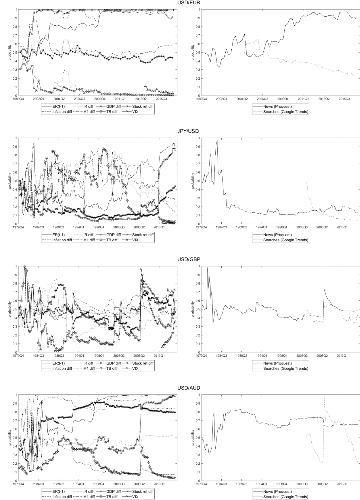
Figure 1. Time-varying posterior probabilities of including predictors into the models.
