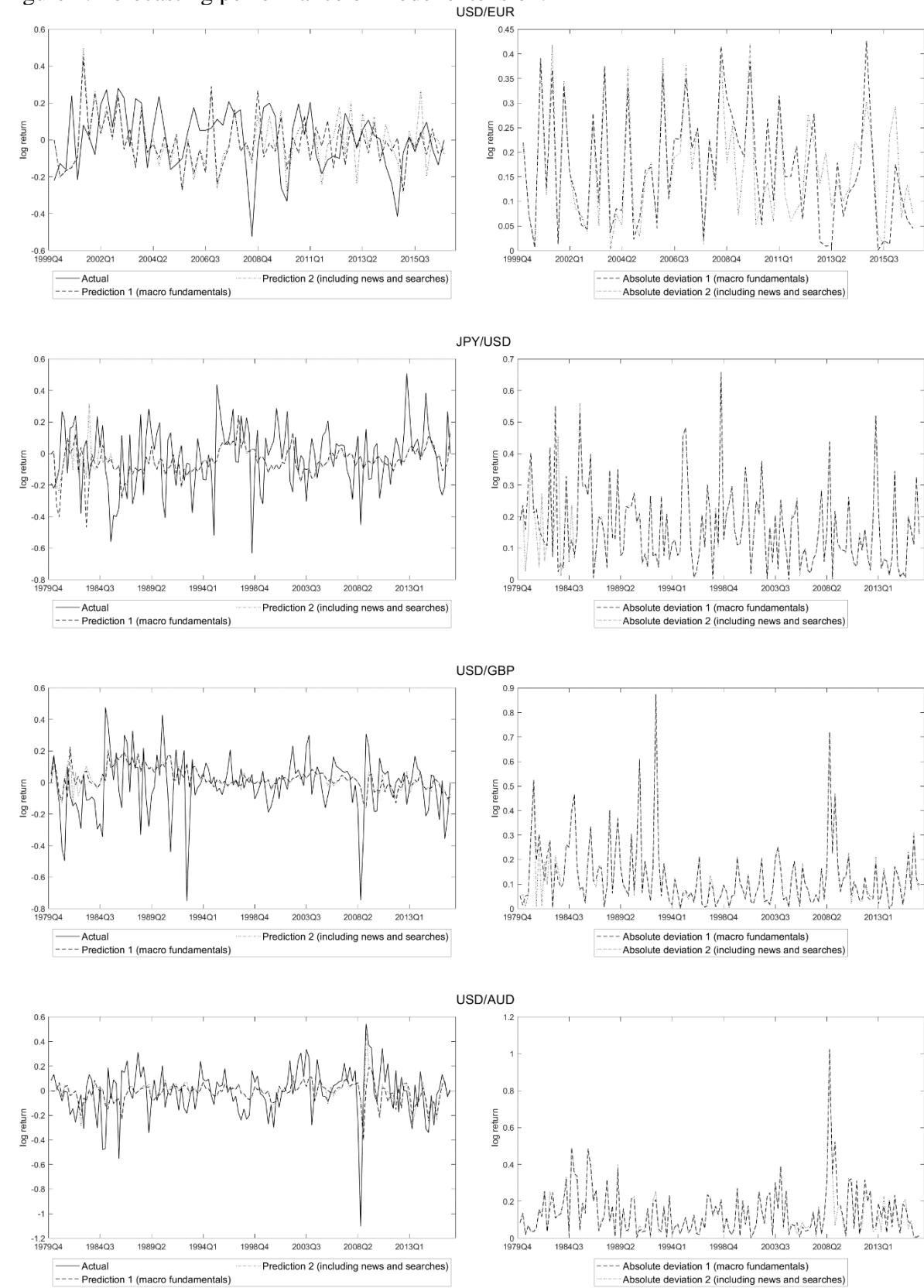
Figure 2. Forecasting performance of model extension.
