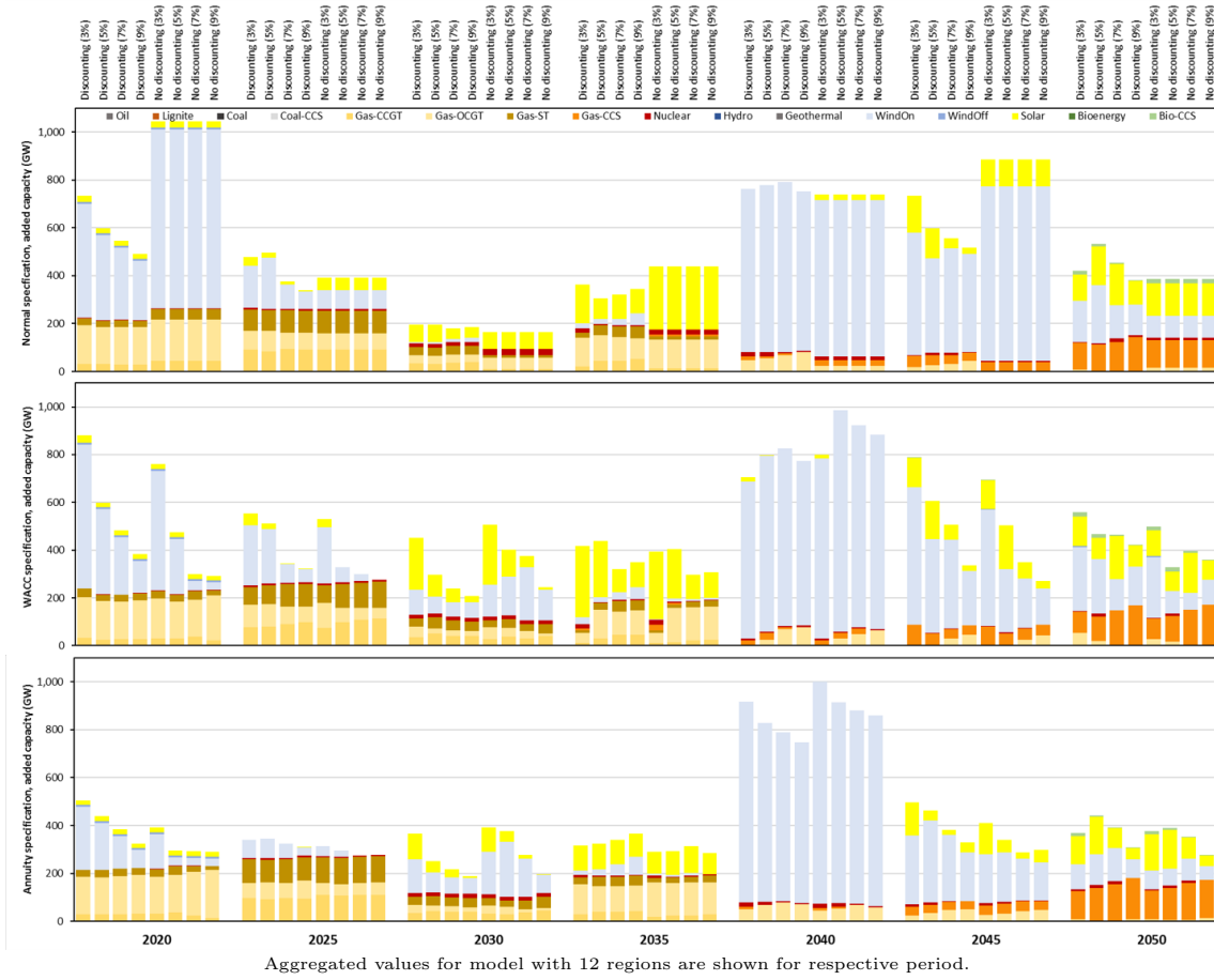
Figure 2: Added capacities for different investment cost specifications
