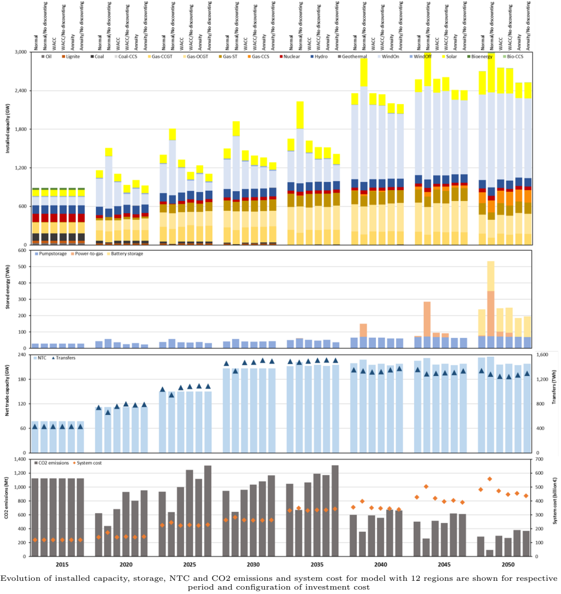
Figure 1: Results for different investment cost specifications
