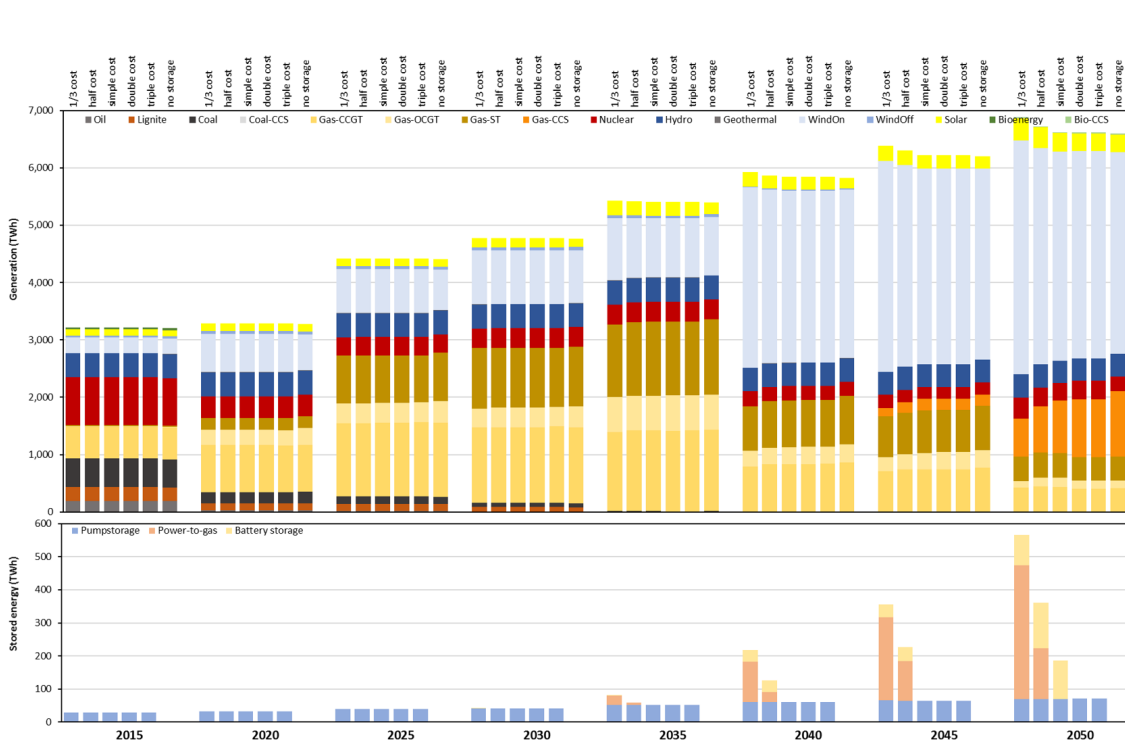
Figure 9: Generation and storage mix for varying storage cost
