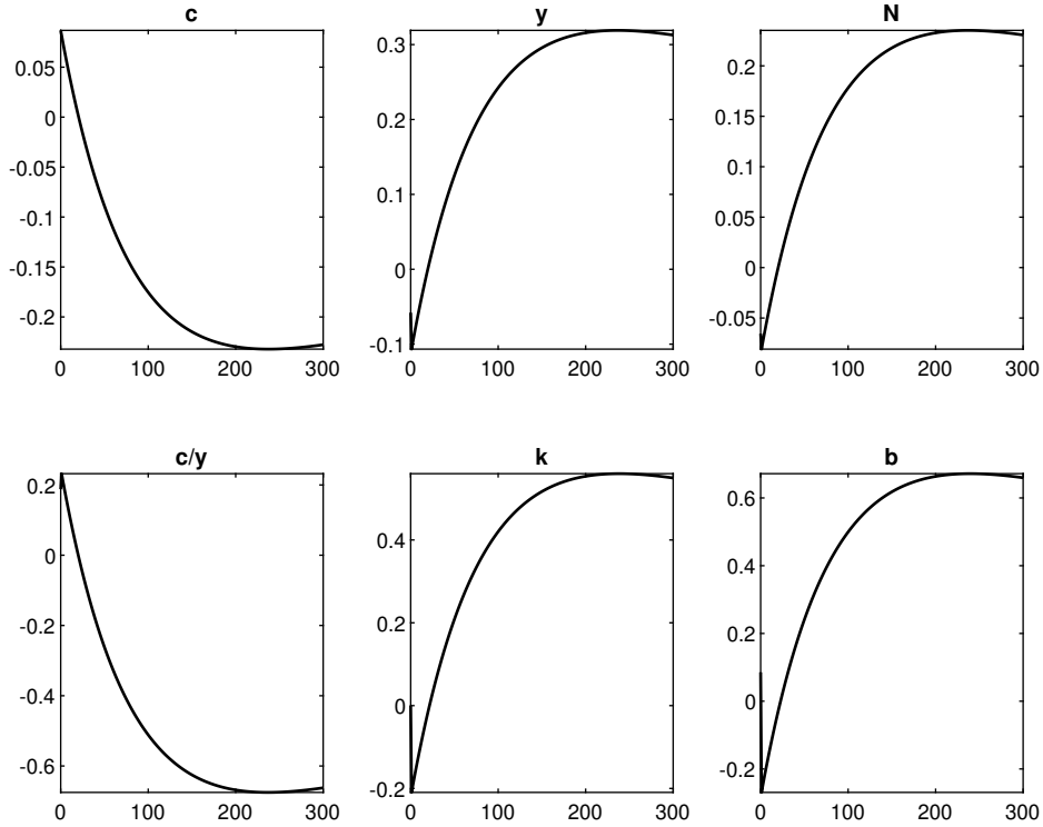
Figure 6: Impulse responses to a one percent increase in the productivity growth shock
