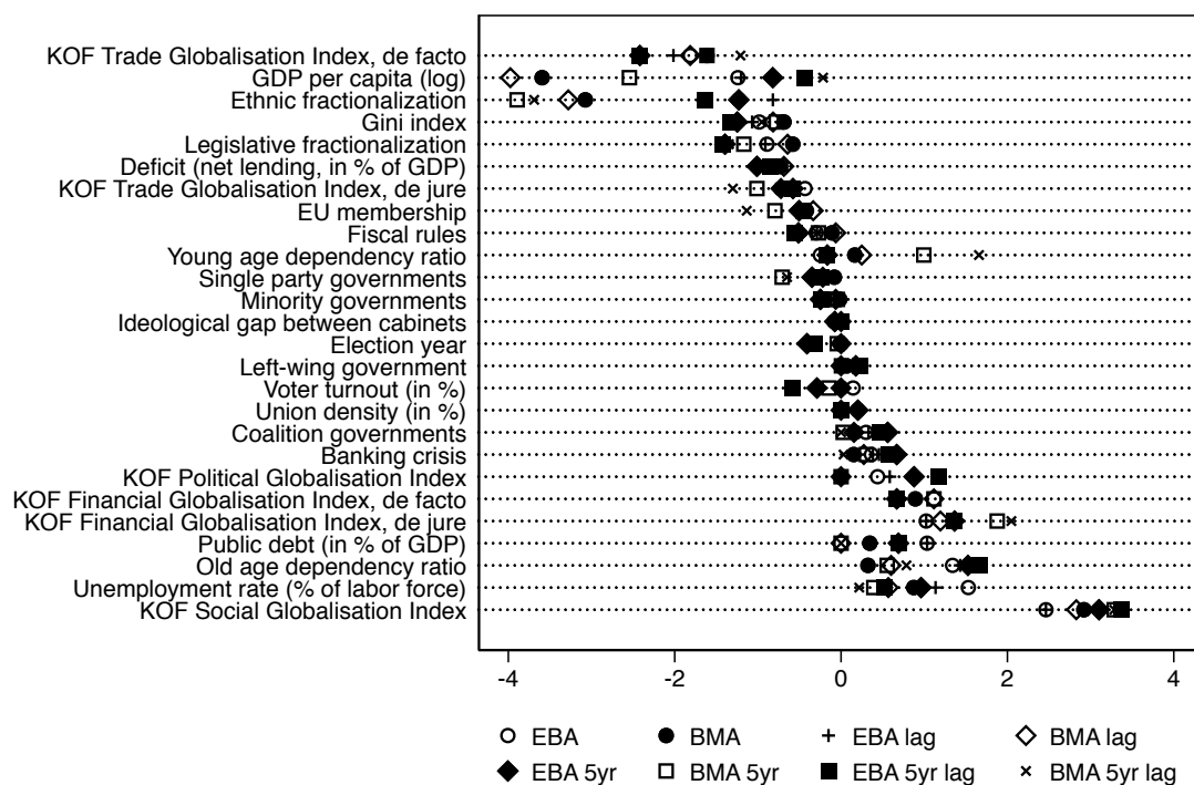
Figure A. 4: Coefficients plot, all determinants
