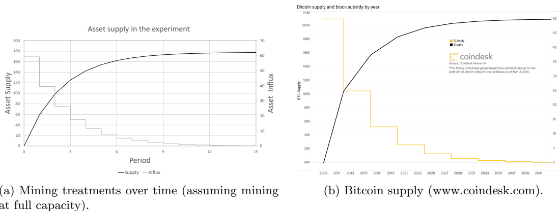
Figure 1: Contrasting asset supply between experimental PoW implementation and Bitcoin.
