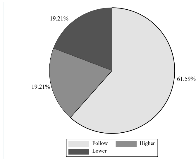
Figure 9: Translation Error
