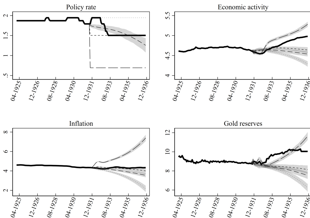
Figure A.6: Simulations based on the baseline 11-Factor VAR for different policy paths
