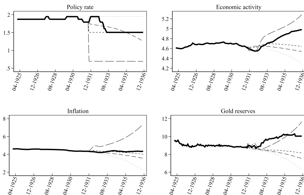
Figure 8: Simulations based on the baseline 11-Factor VAR for different policy paths
