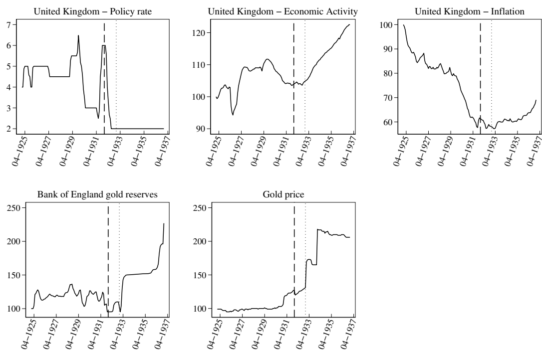
Figure 7: Global factors, April 1925 – December 1936.
