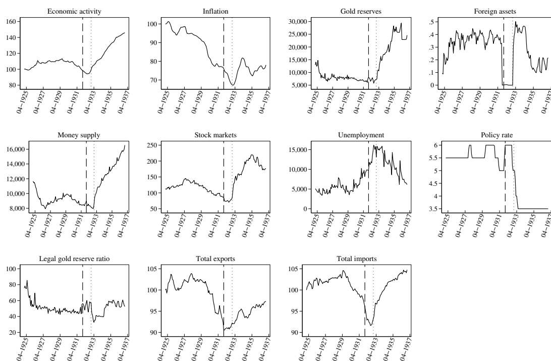
Figure 6: Domestic factors, April 1925 – December 1936.
