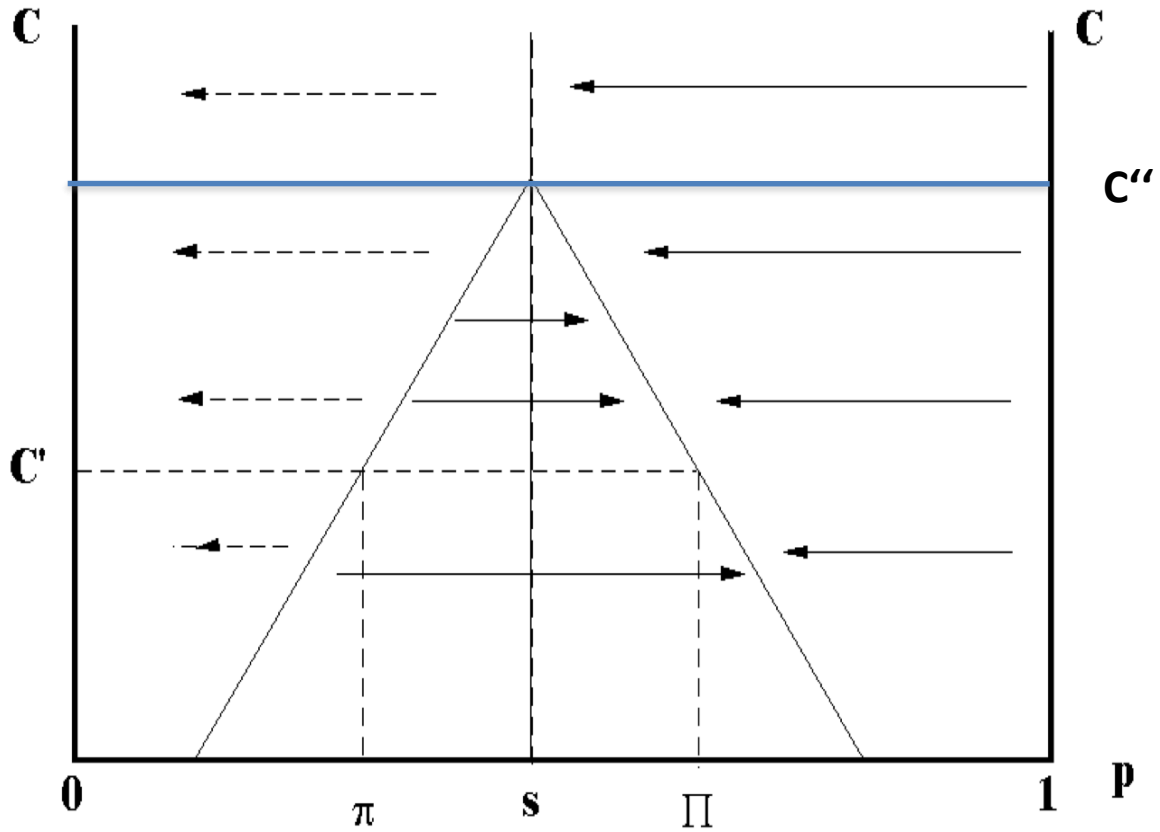
Figure 2 Evolution of population share p of committed actors for alternative levels of cost and given reliability of type detection
