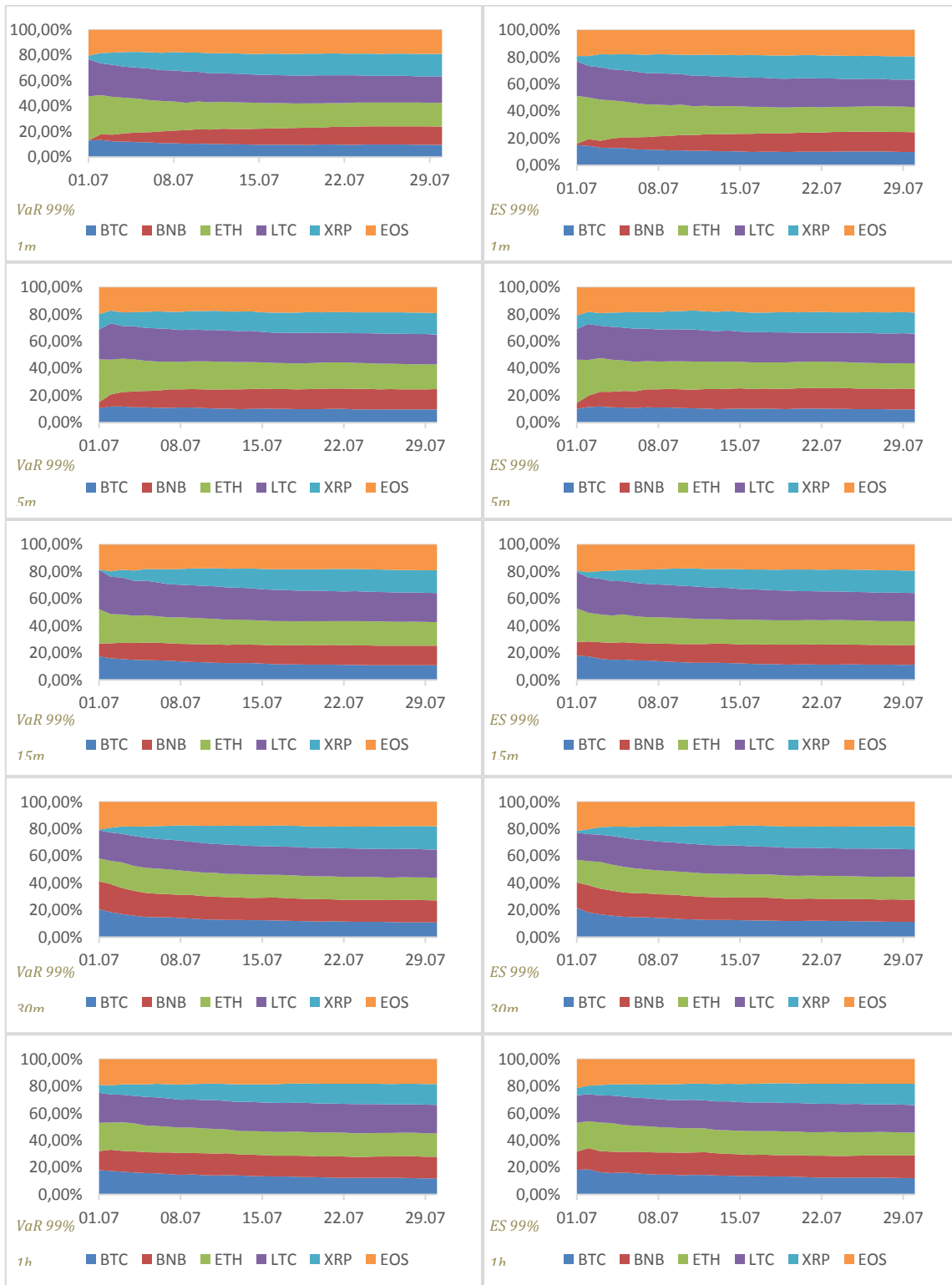
Figure 4.4. Constant Kernel marginal tail risk allocations 99%
