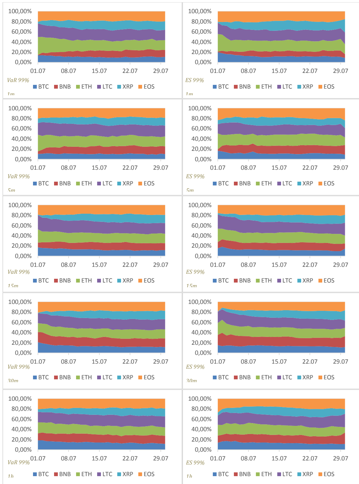
Figure 4.6. Linear Kernel marginal tail risk allocations 99%
