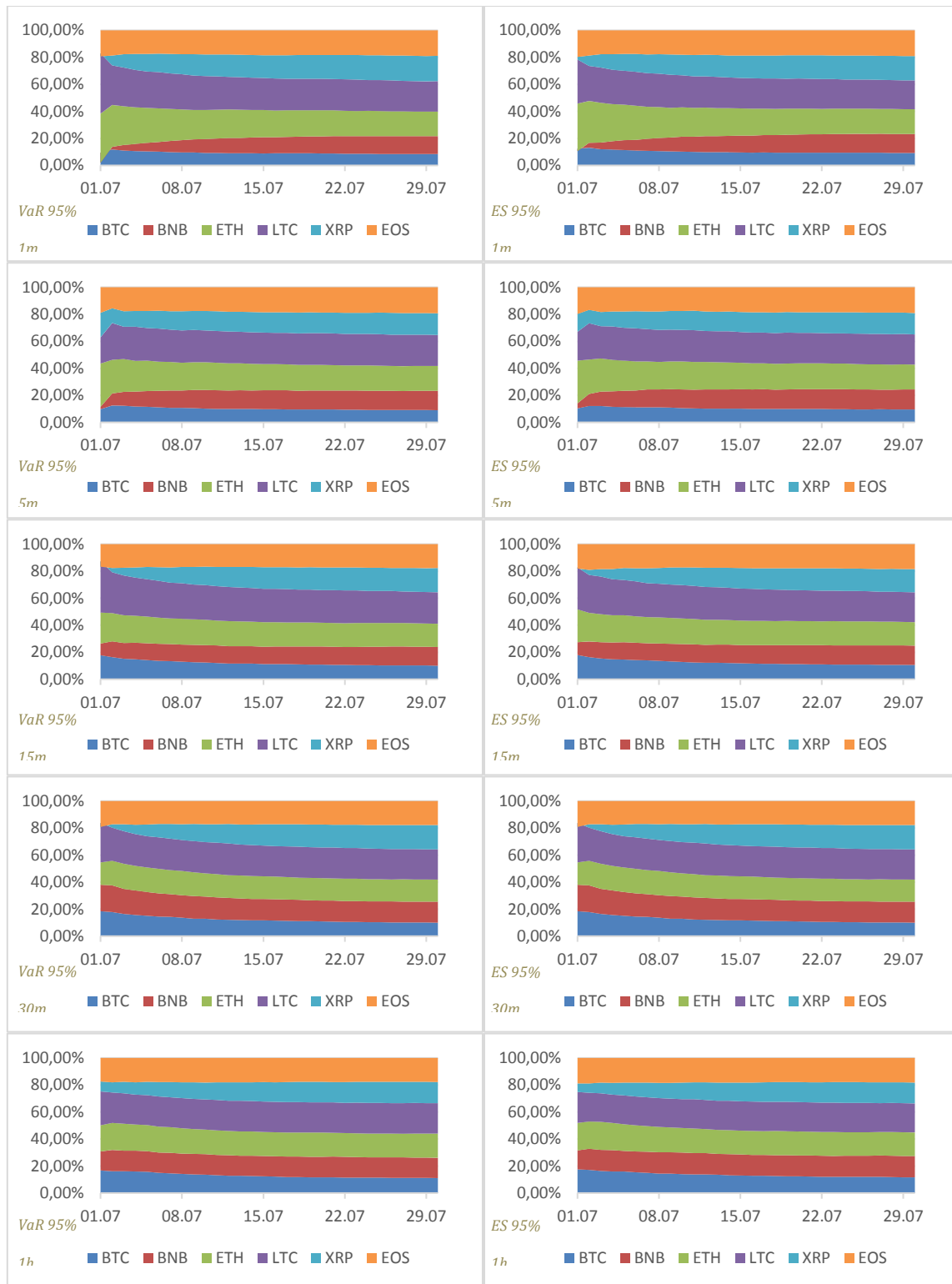
Figure 4.5. Constant Kernel marginal tail risk allocations 95%
