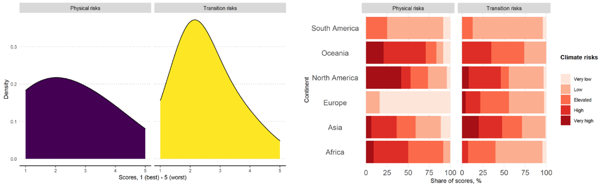
Figure 2: Density plots of climate country scores and share of scores per continent
