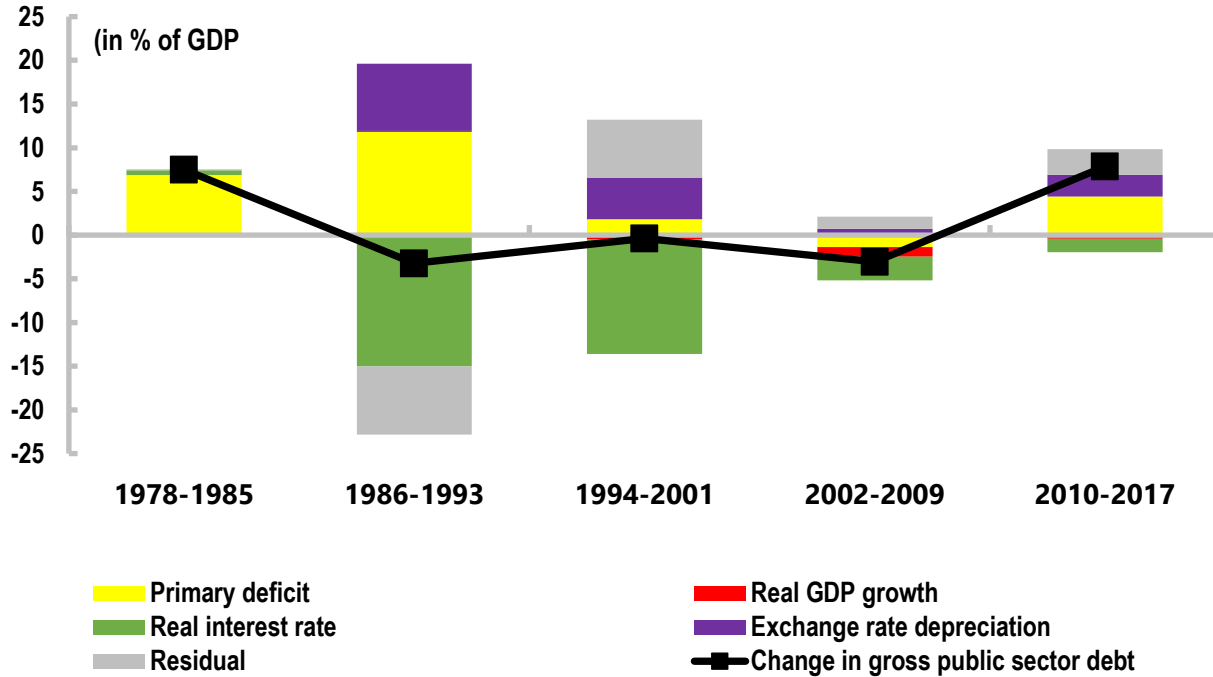
Figure 2. Evolution of Total Debt
