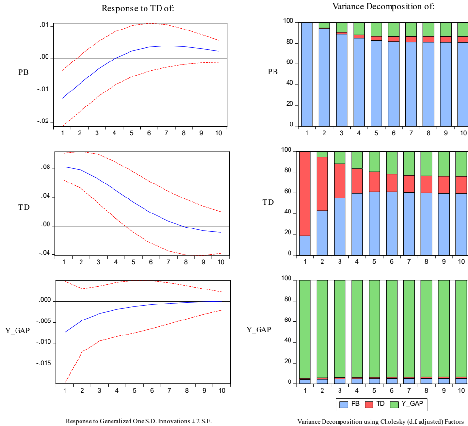
Figure 3. Impulse Response and Variance Decomposition
