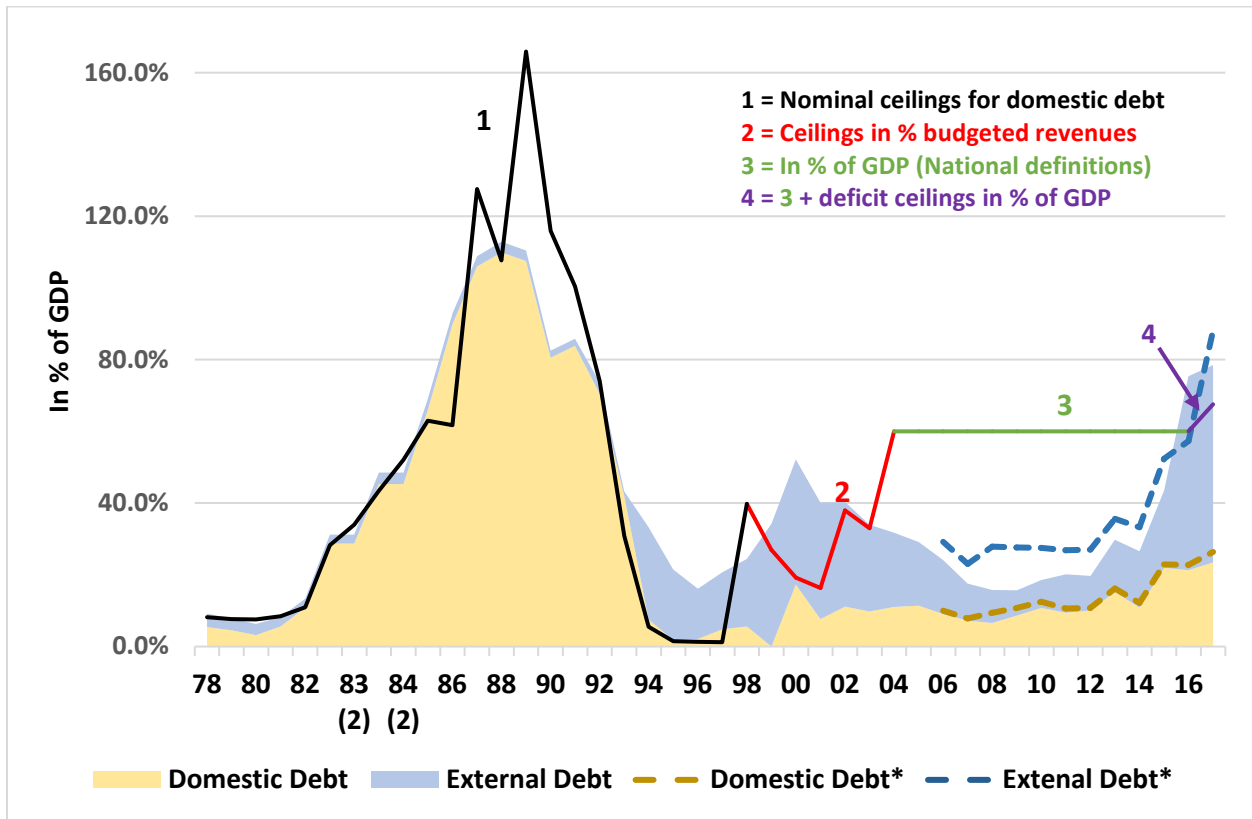
Figure 1. Government Debt and Debt Ceilings 1
