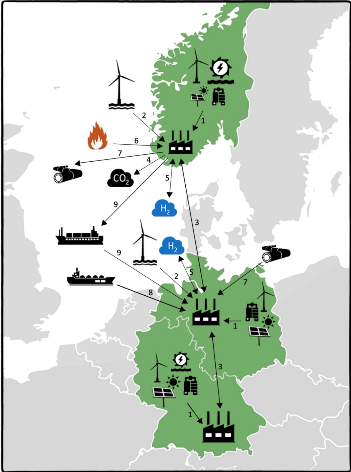
Figure 1: A graphical summary of the different transmission, import and export elements included in the model. Germany is modelled as separate Northern and Southern regions. The numbers are explained in Table 2.
