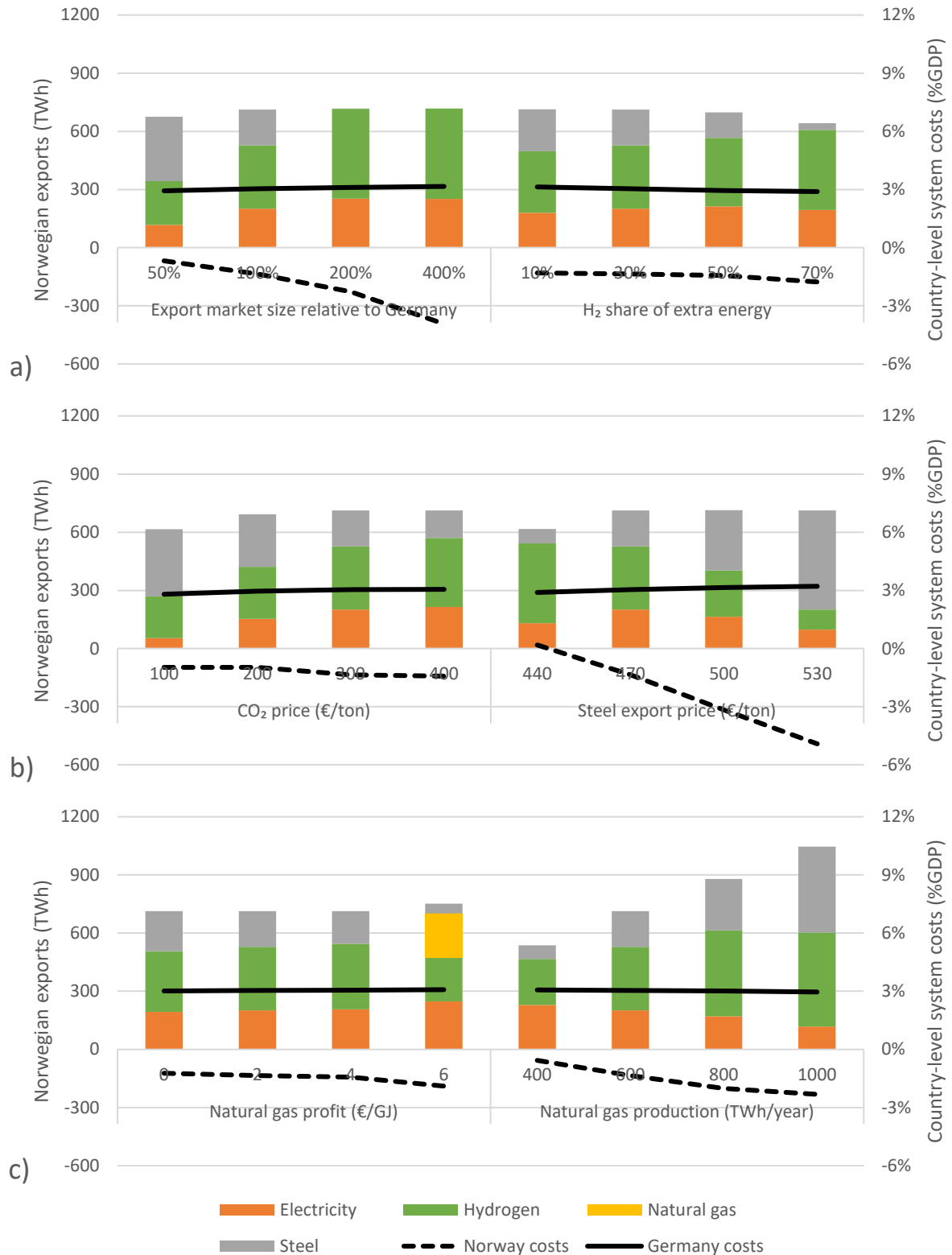
Figure 4: Norwegian exports and country-level costs for various sensitivity scenarios. Norway exports electricity and hydrogen to Germany (limited demand), and steel and natural gas to the global market (unlimited demand). Steel trade flows are presented in energy equivalent terms: 2.79 MWh of hydrogen and electricity per ton of steel.
