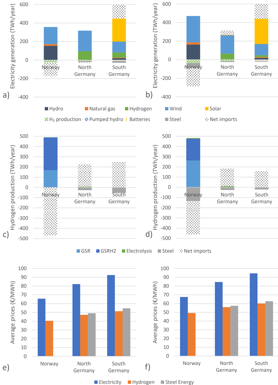
Figure 2: Various results from the baseline scenario without (panels a, c, e) and with (panels b, d, f) steel trade. Steel exports in panels b and d are presented in energy-terms by accounting for 2.04 MWh of hydrogen and 0.75 MWh of electricity per ton of steel. Similarly, the Steel Energy price in panels e and f is calculated as the steel price (€/ton) minus steel production CAPEX and OPEX (levelized to €/ton) divided by 2.79 MWh/ton (combined hydrogen and electricity needed per ton of steel).
