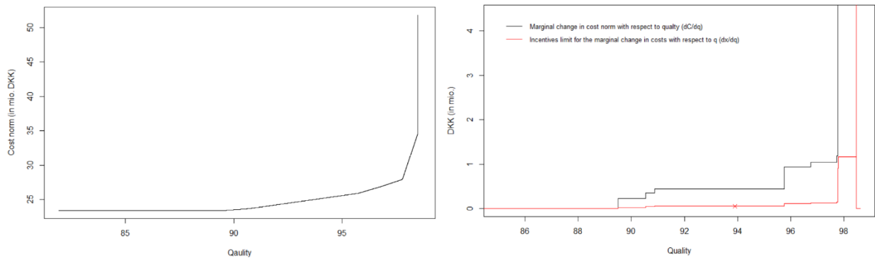
Figure 4-1 Relationship between quality, cost norm, marginal changes in cost norm, and marginal quality cost
