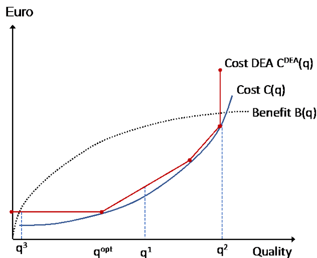
Figure 2-3 Using a DEA-based revenue cap
