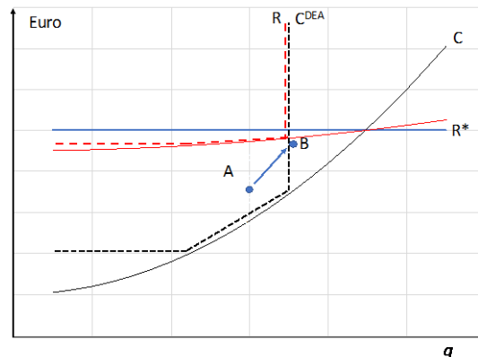
Figure 3-2 Illustrative example with DEA-based cost norms
