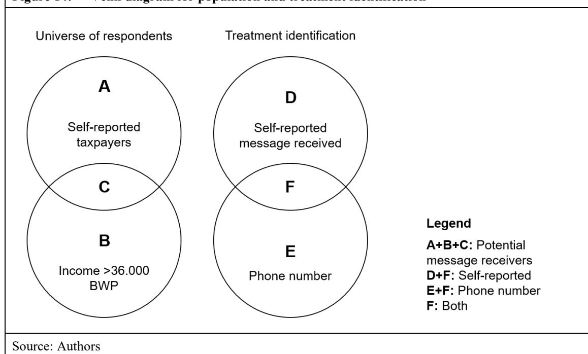
Figure 14: Venn diagram for population and treatment identification
