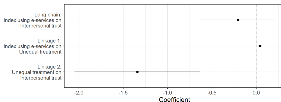
Figure 12: Rope ladder estimates equal treatment hypothesis
