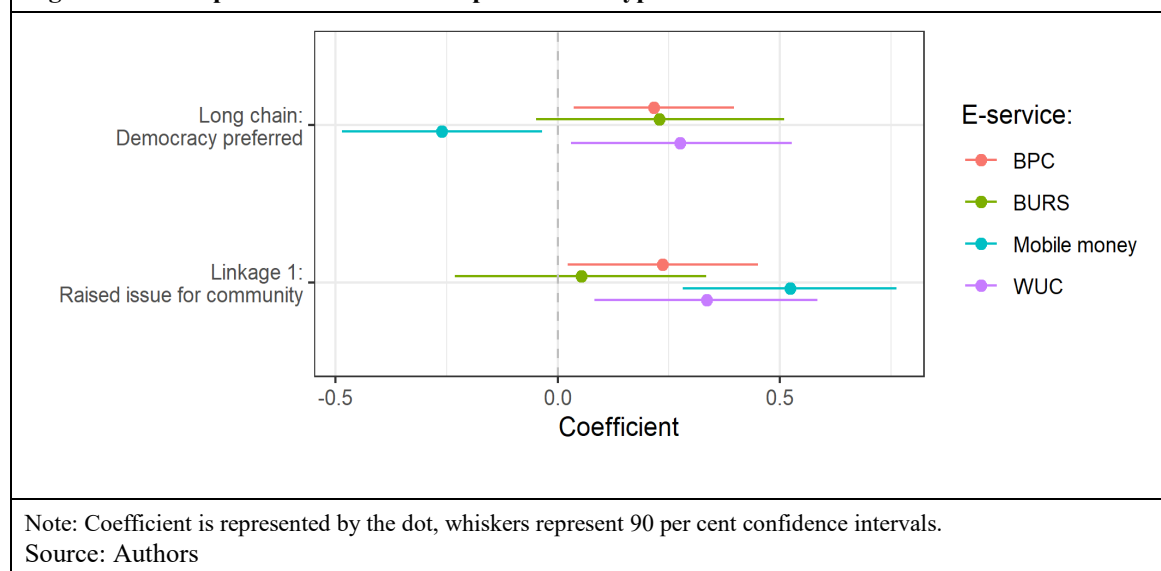
Figure 9: Rope ladder estimates empowerment hypothesis individual services
