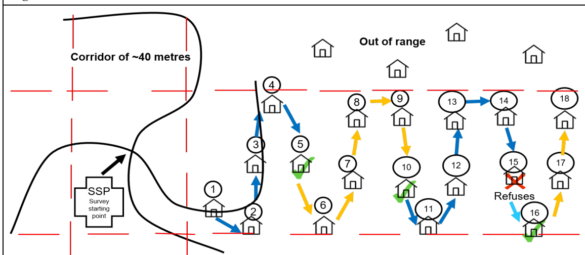
Figure 6: Random walk in the case of scattered houses
