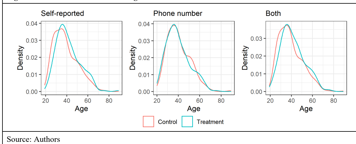
Figure 15: Visual balance check age
