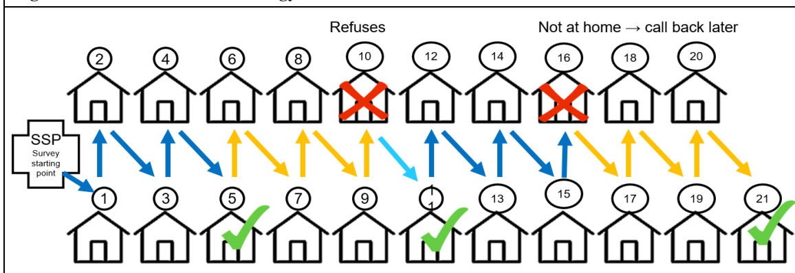
Figure 5: Random walk strategy
