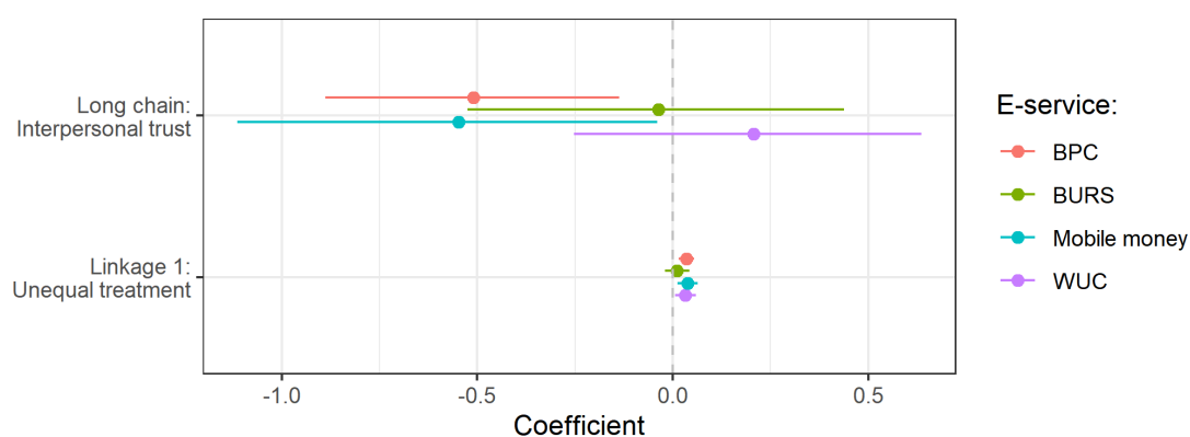
Figure 13: Rope ladder estimates equal treatment hypothesis individual services
