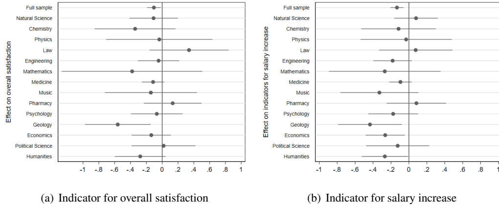
Figure 11: Effect on course SET of online teaching due to the COVID-19 pandemic, courses not changed (controls added)
