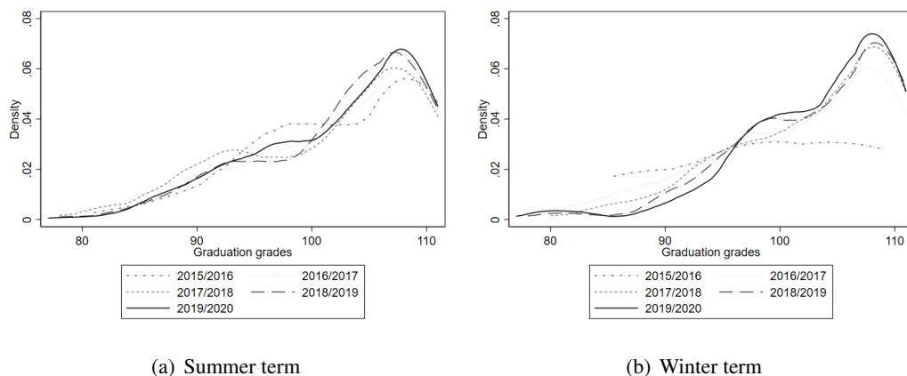
Figure 9: Density of graduation grades over time
