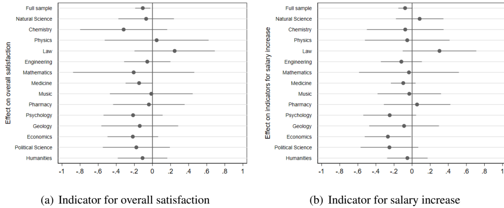
Figure C.10: Effect on course SET of online teaching due to the COVID-19 pandemic, multiple pre-treatment periods (no controls added)
