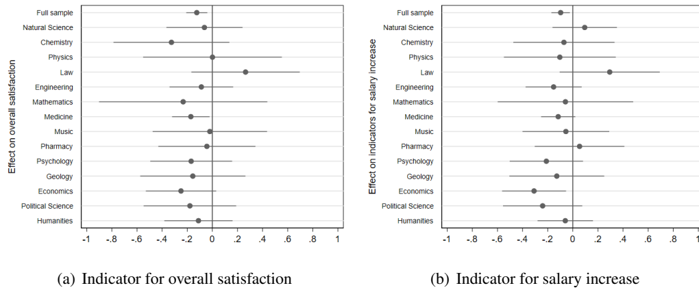
Figure 17: Effect on course SET of online teaching due to the COVID-19 pandemic, multiple pre-treatment periods (controls added)
