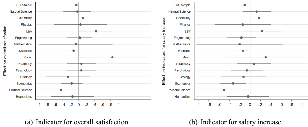
Figure C.8: Effect on course SET of online teaching due to the COVID-19 pandemic, mandatory courses (no controls added)
