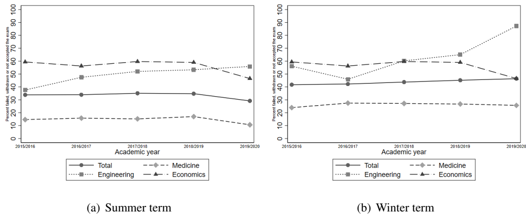
Figure 10: Percentage of exams failed over time, full sample and selected departments
