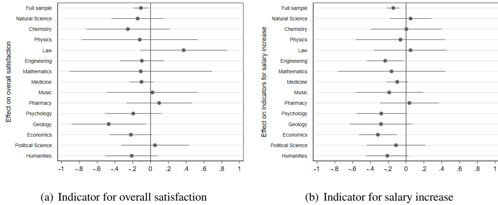
Figure 4: Effect on course SET of online teaching due to the COVID-19 pandemic, full sample (no controls added)
