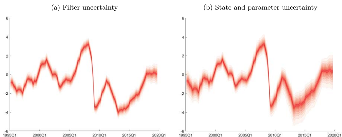
Figure 6: State and parameter uncertainty around the euro area output gap estimate (model A)
