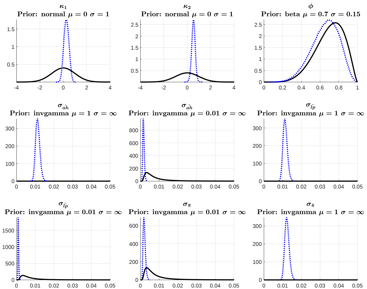
Figure B2: Prior and marginal posterior distribution of the parameters (model A)
