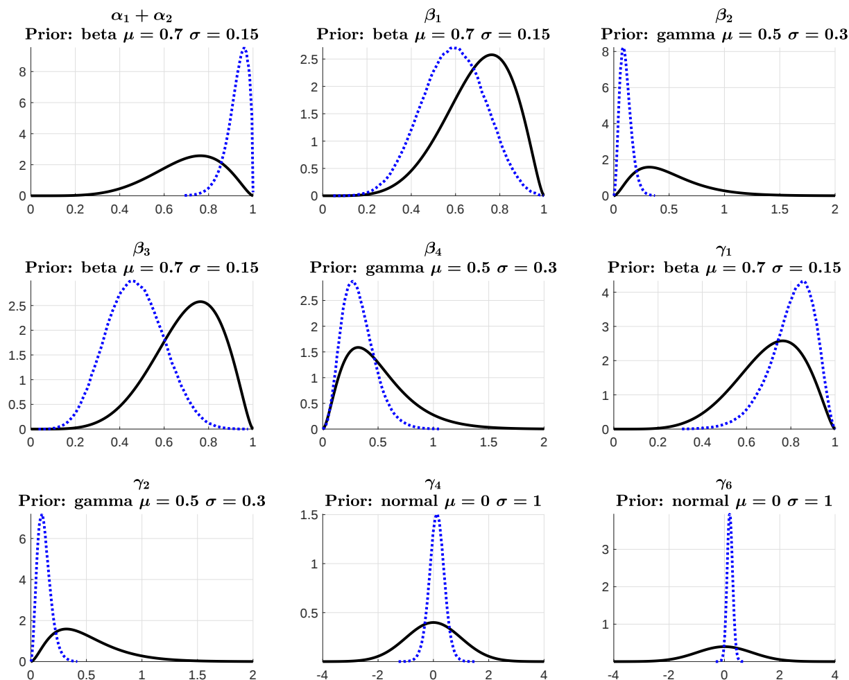
Figure B1: Prior and marginal posterior distribution of the parameters (model A)
