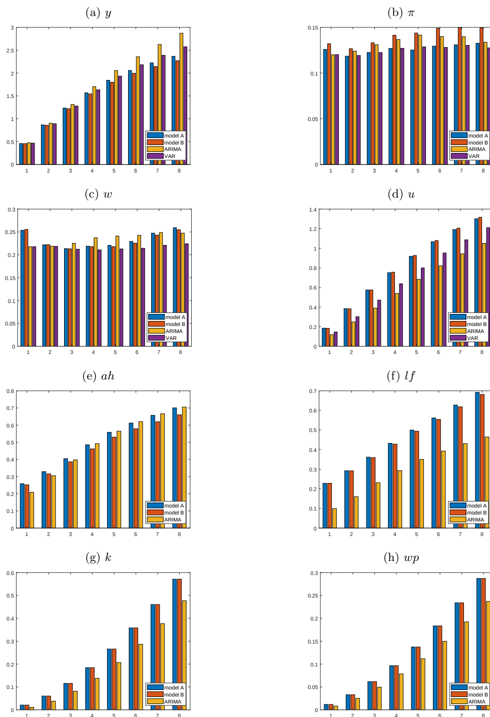
Figure C1: RMSFEs with fixed parameters
