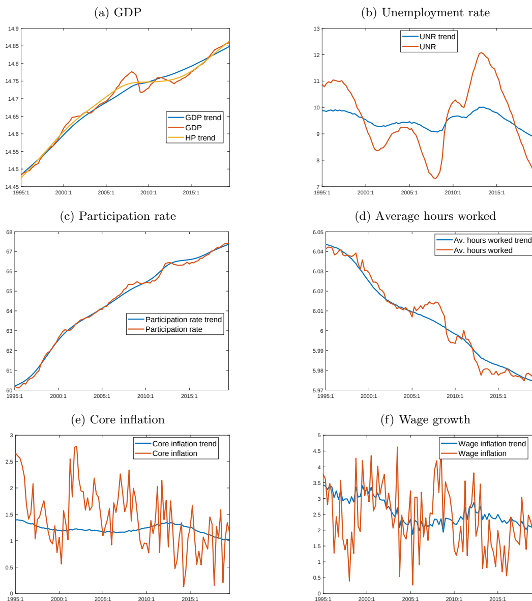
Figure 4: Key variables and their trends as estimated in Model B
