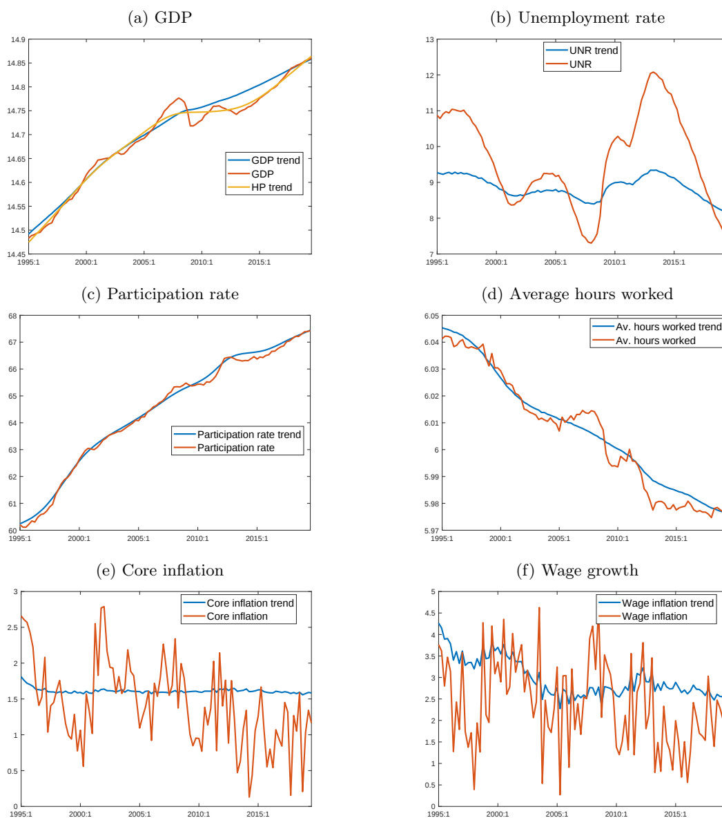
Figure 2: Key variables and their trends as estimated in Model A
