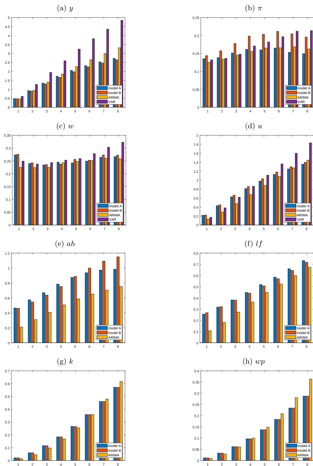
Figure C2: RMSFEs with re-estimated parameters
