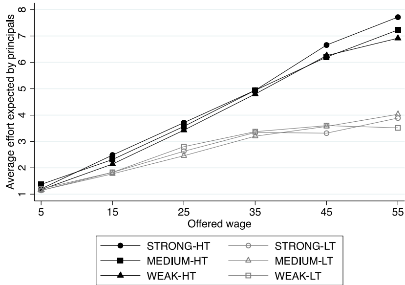
Figure 2: Manipulation Check
