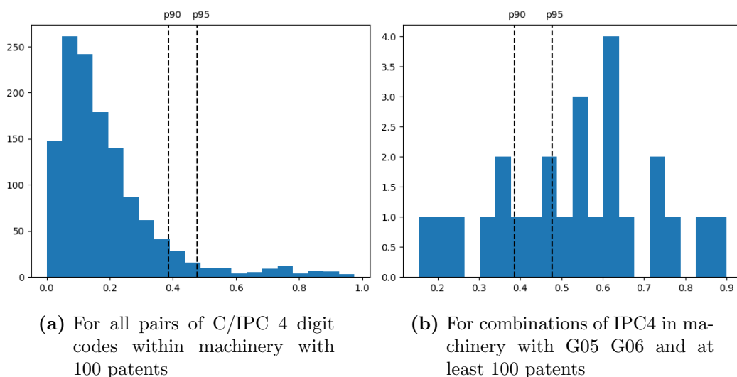
Figure A.4: Histograms of the prevalence of automation keywords. The p90 and p95 lines are those of the 6 digit distribution and mark the thresholds used to define auto90 and auto95 technological categories.
