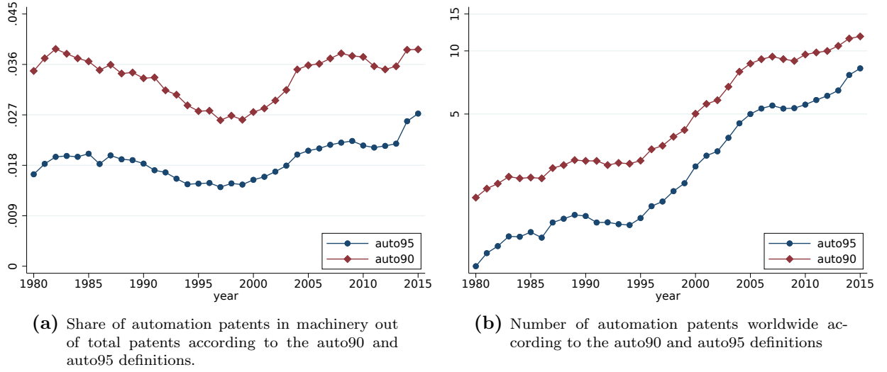
Figure A.3: Trends in automation (for biadic applications)
