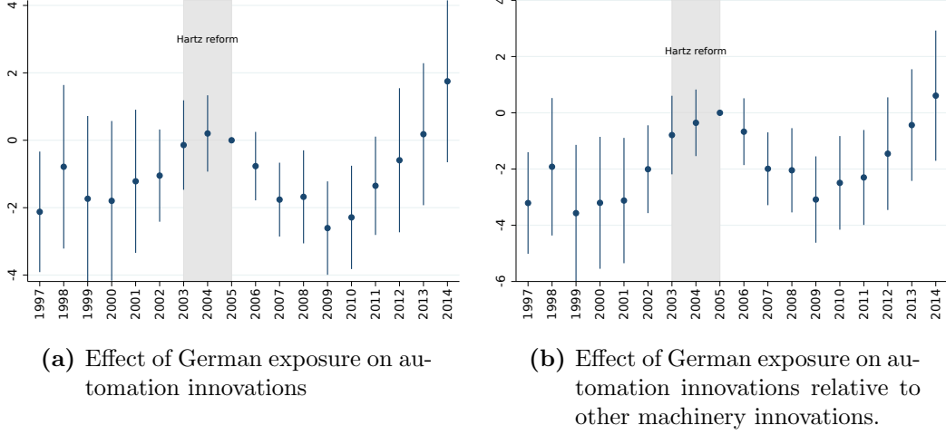
Figure 5: Effect of German exposure on automation innovations. Panel (a) reports coefficients on the interaction between the German weight and a set of year fixed effects in a Poisson regression of auto95 innovations controlling for a full set of fixed effects and firm innovation stocks with 2153 firms. Panel (b) reports coefficients on the triple interaction between the German weight, a dummy for auto95 innovations and a set of year fixed effects in a Poisson regression of auto95 and other machinery innovations controlling for a full set of fixed effects, firm innovation stocks and the interaction between the German weight and a set of year fixed effects with 6452 firms.
