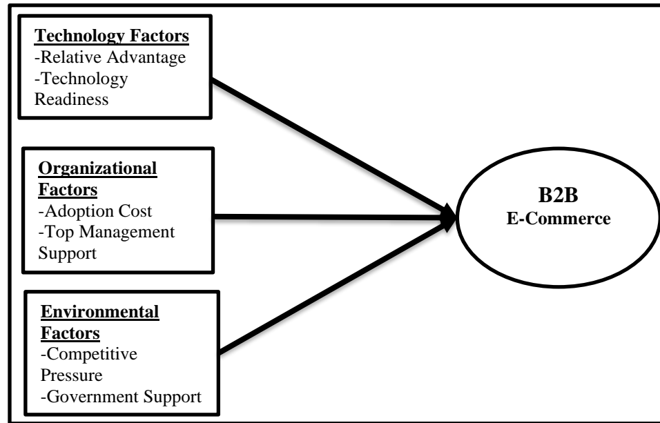
Figure 1: Research Framework
