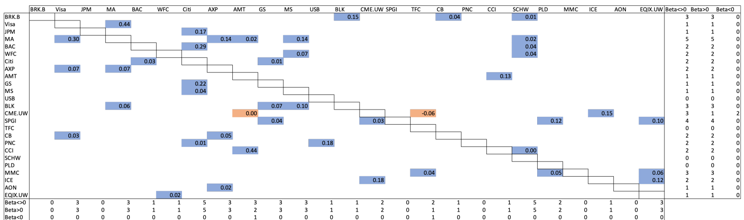
Figure 3.12: Network on 20200203 for \tau = 0.25
