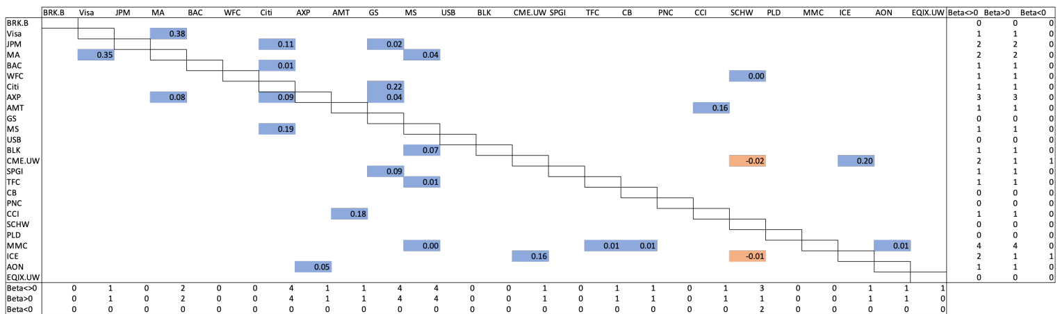
Figure 3.13: Network on 20200203 for \tau = 0.5
