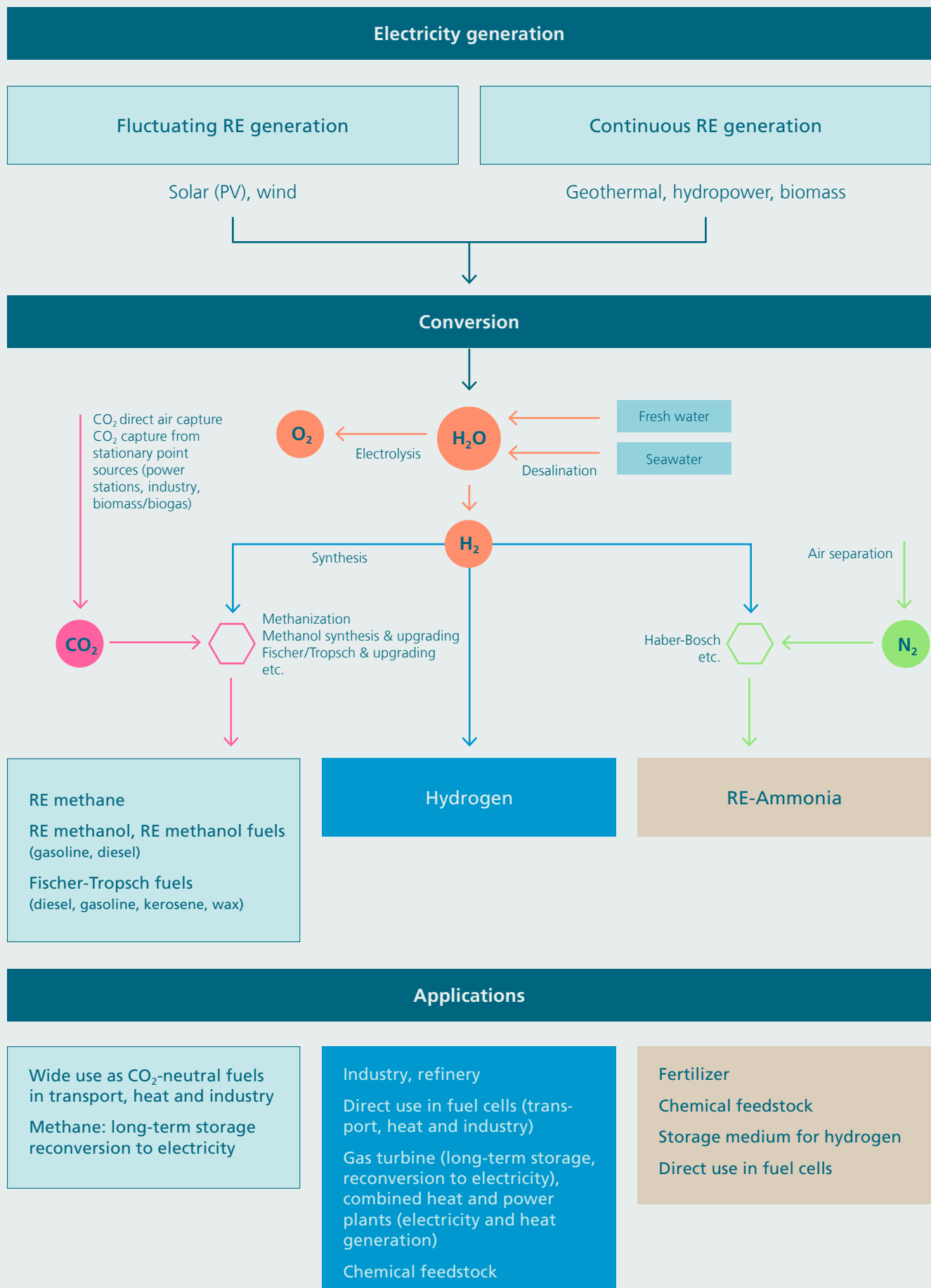
Figure 1: Selected conversion paths to produce green hydrogen and synthesis products based on renewable electricity (as an extension of [4])
