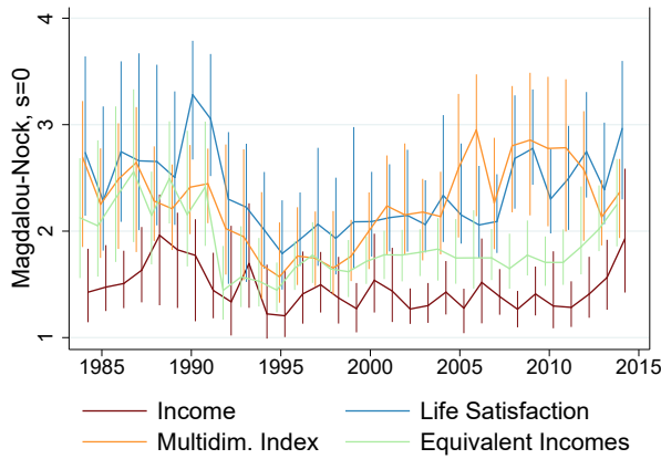
(a) Magdalou-Nock, s = 0
