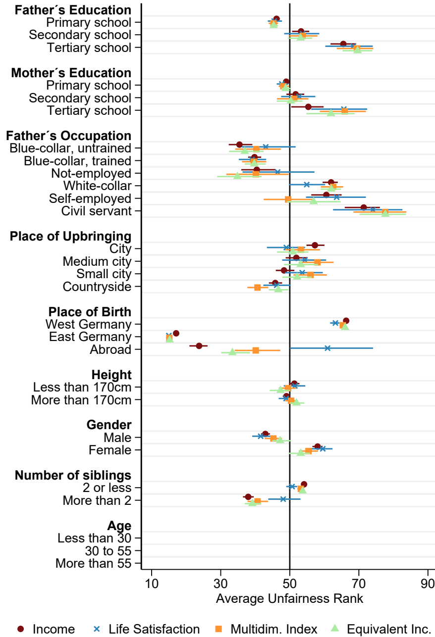
Figure 3.5: Changing the Responsibility Cut: \text{Effort} = \{4\text{var}, \text{residual}, \text{cor}, \text{age}, \text{pref}\}
