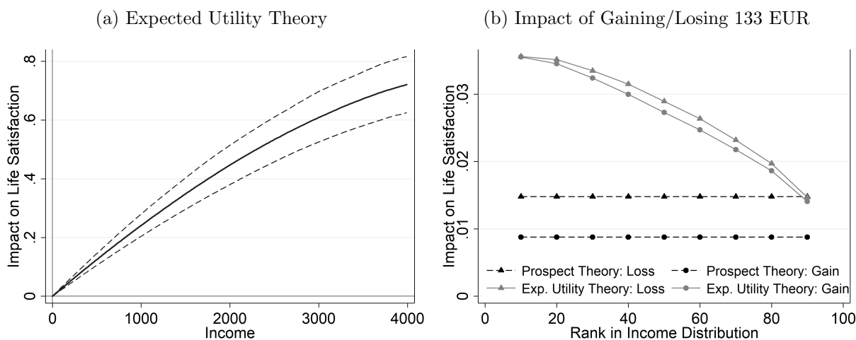
Figure 2.8: Testing H3
