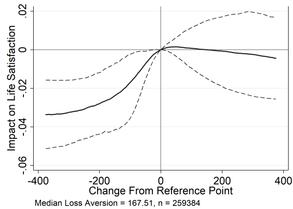
(c) Spline with 6 Knots
