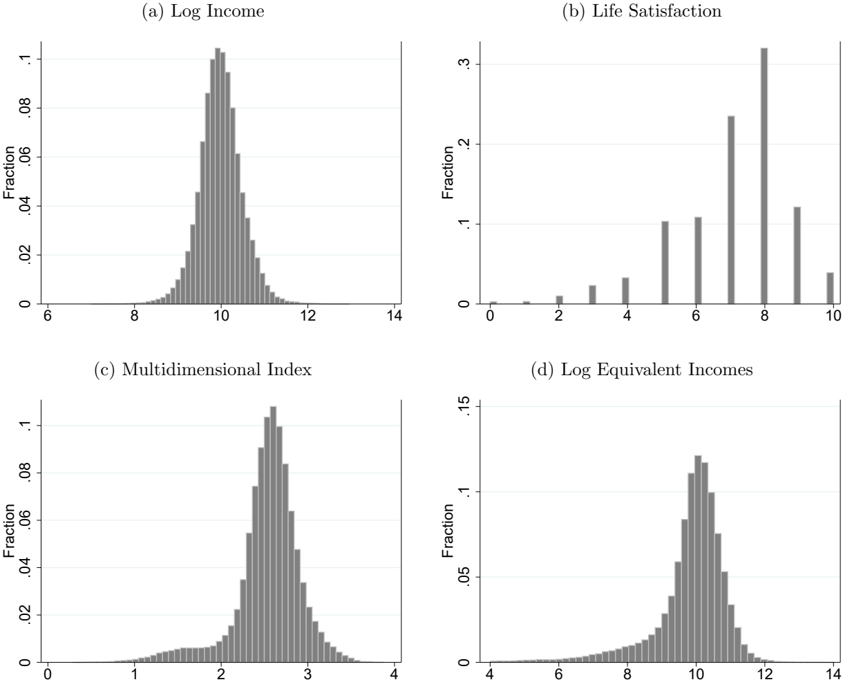
Figure 3.1: Histograms
