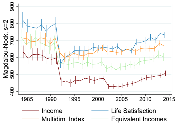
(c) Magdalou-Nock, s = 2
