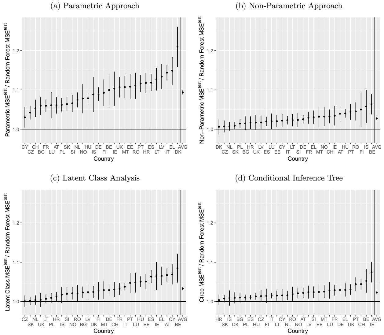
Figure 4.6: Comparison of Models' Test Error
