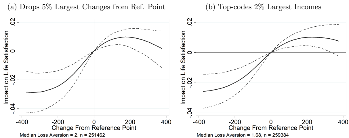
Figure 2A.7: Outliers
