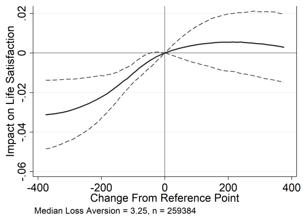
(b) Spline with 5 Knots
