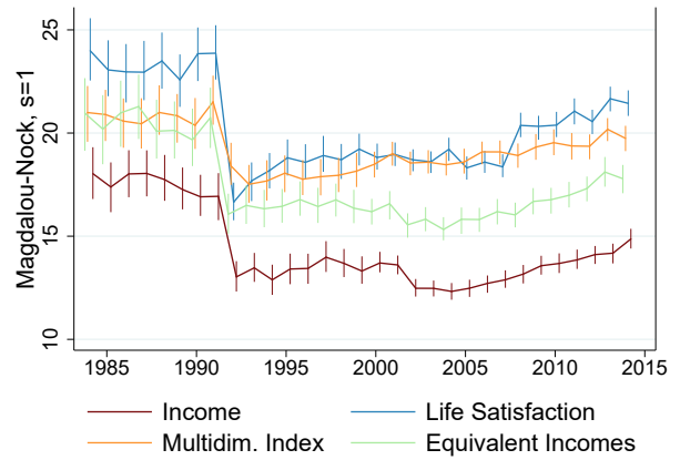
(b) Magdalou-Nock, s = 1
