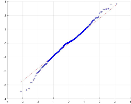
(f) QQ-plot of residuals
