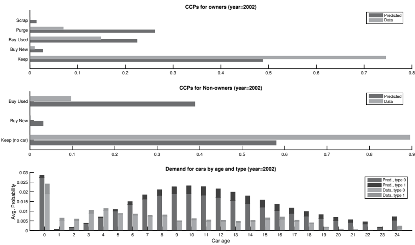
Figure E.1: Model Fit: Conditional Choice Probabilities
