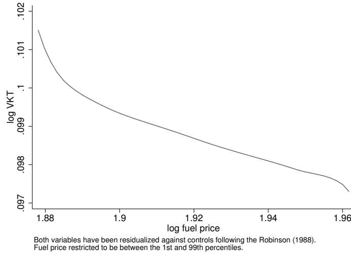
Figure 7.1: Semi-parametric demand curve
