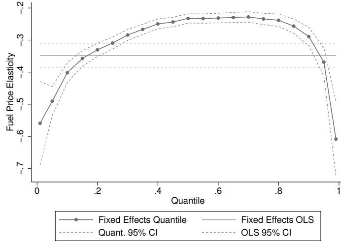
Figure 5.1: Elasticity by Conditional Quantile
