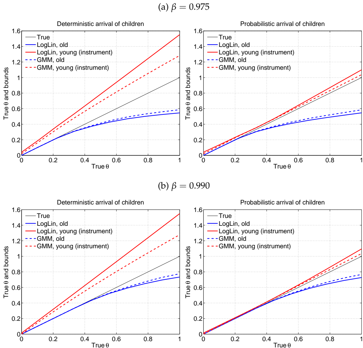
Figure 6 – Bounds, \beta = \{0.975, 0.99\} .
