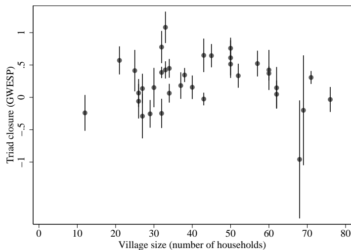
Figure 3: Triad closure (GWESP) coefficient: full model
