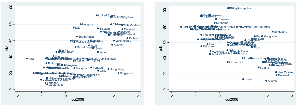
Figure 2. Simple plot of cci2006 vs IDV and cci2006 vs PDI (79 countries).
