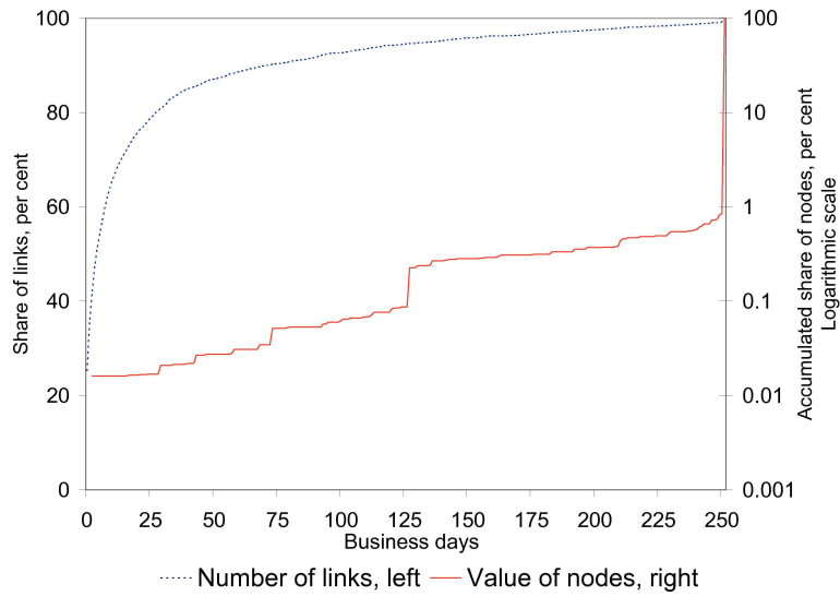
Figure 3.7: Frequency of links and nodes
