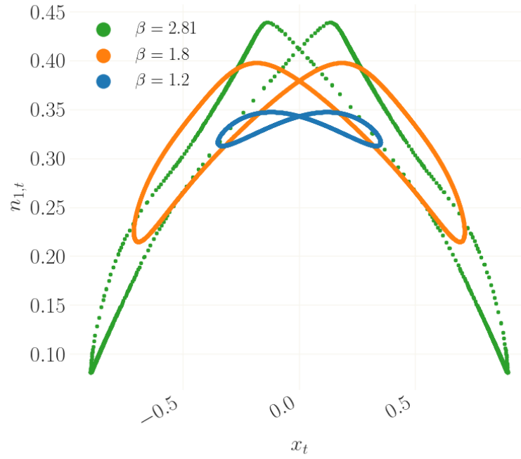
Figure C.21: Phase plot in (x_t, n_{1,t}) -space for different values of \beta corresponding to the bifurcation diagram with limit cycles in Figure 3 (based on policy function iteration).
