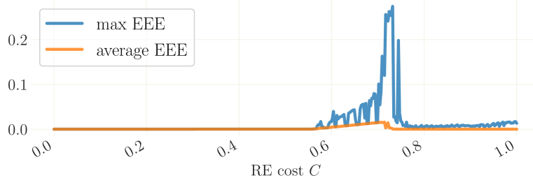
Figure B.17: Average and maximum absolute Euler equation errors for the bifurcation w.r.t. the cost parameter C as in Figure 7 but when using policy function iteration.
