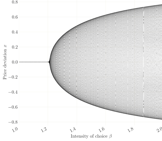
Figure 2: Bifurcations w.r.t. the intensity of choice \beta . Figure 3: Bifurcations w.r.t. bias b . All other parameters as in Table 2. Required minimal precision is \epsilon = 1e - 14 .
