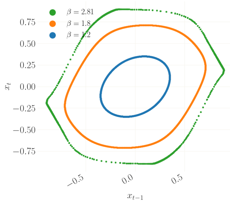
Figure C.23: Phase plot in (x_{t-1}, x_t) -space for different values of \beta corresponding to the bifurcation diagram with limit cycles in Figure 3 (based on policy function iteration).
