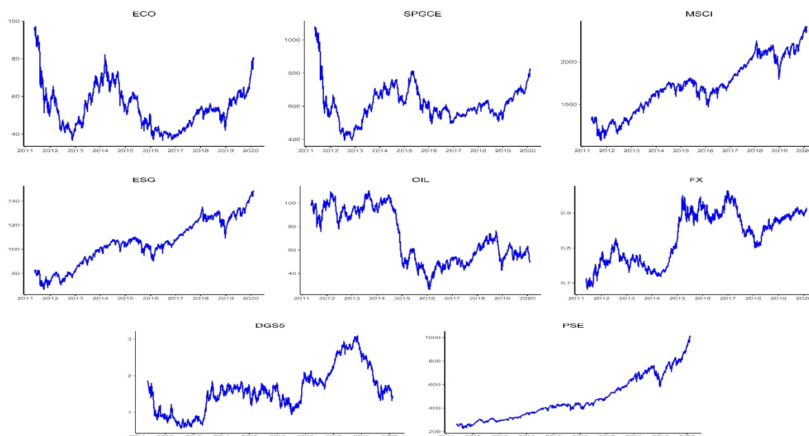
Figure 3. Historical prices (level)
